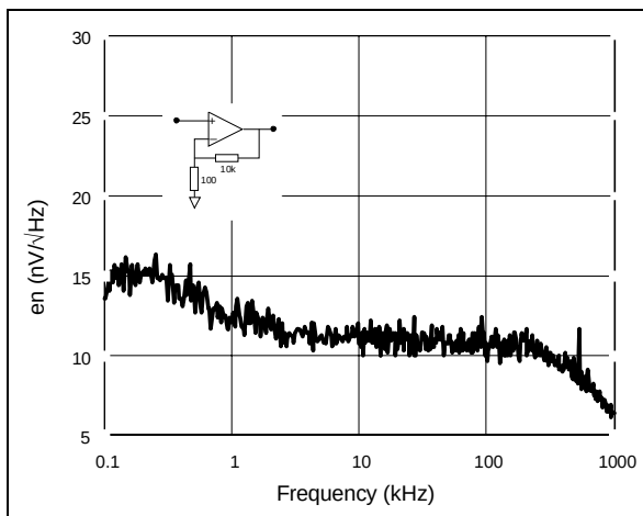
Equivalent Noise Voltage Gain=100, V_{CC}=\pm 5V , No load
