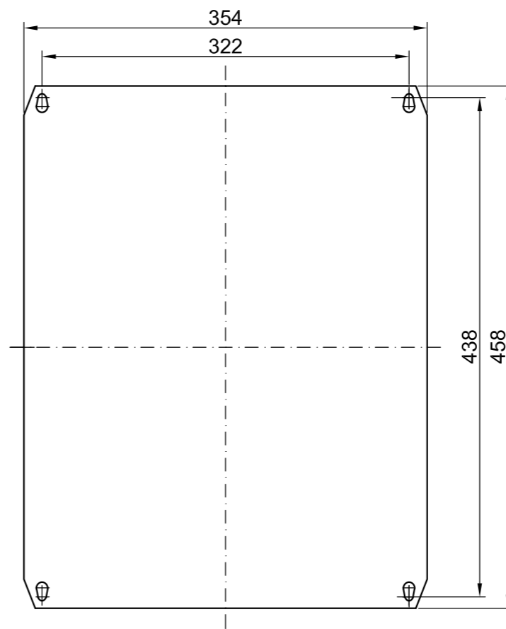
Base Plate
