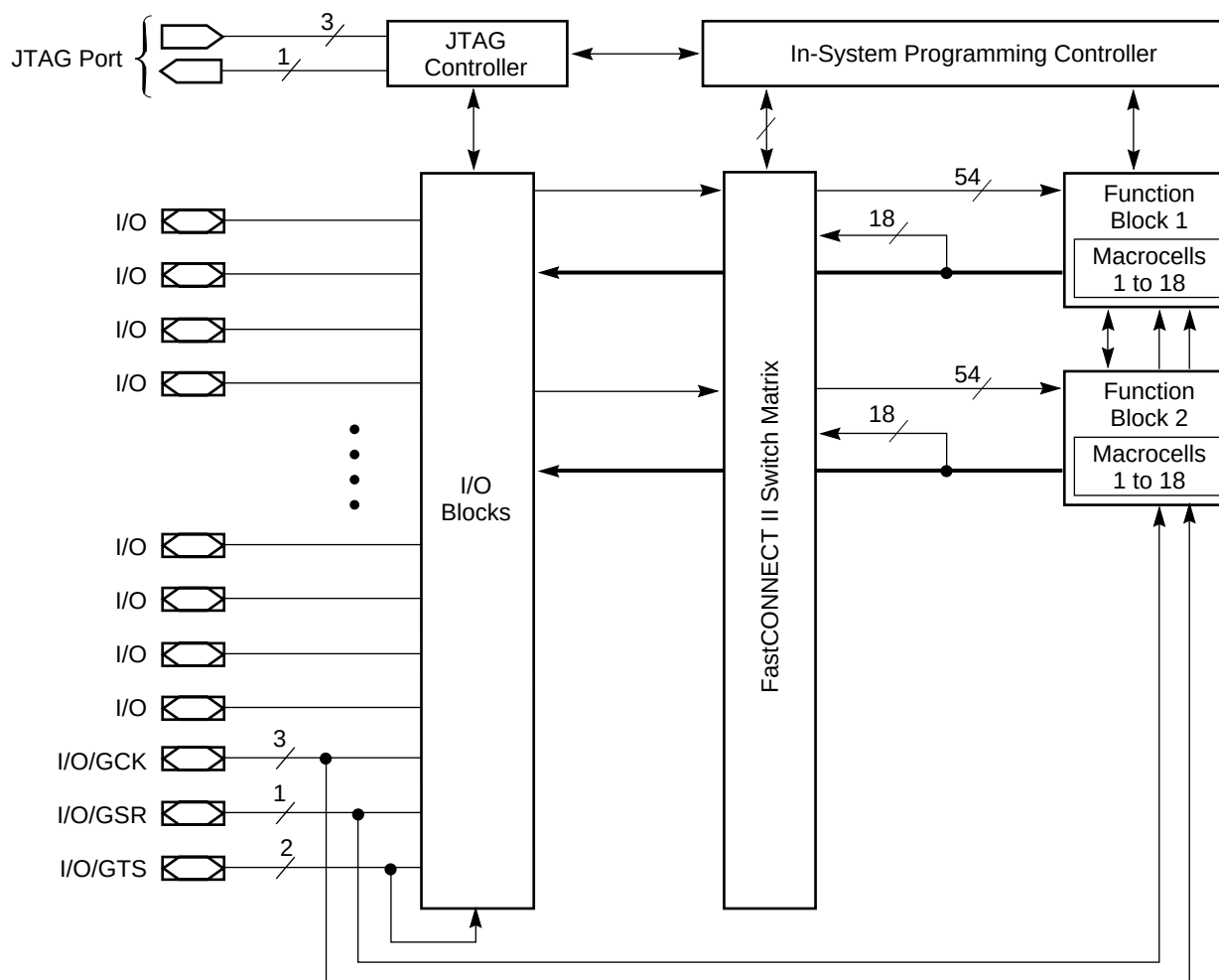
Figure 2: XC9536XL Architecture
