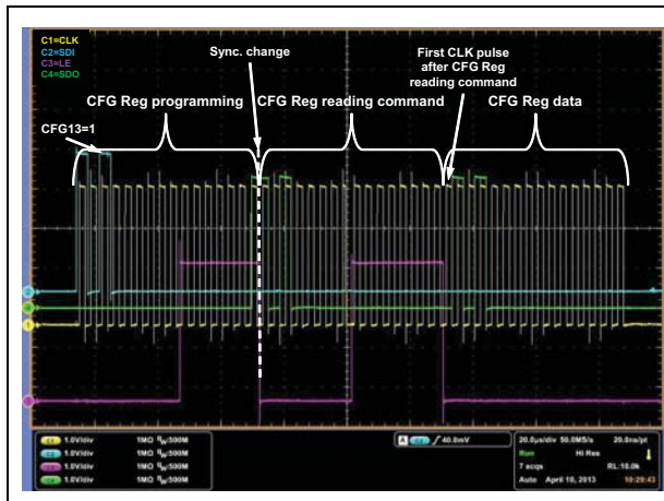
Figure 15. Configuration register reading sequence - SDO delay activates
