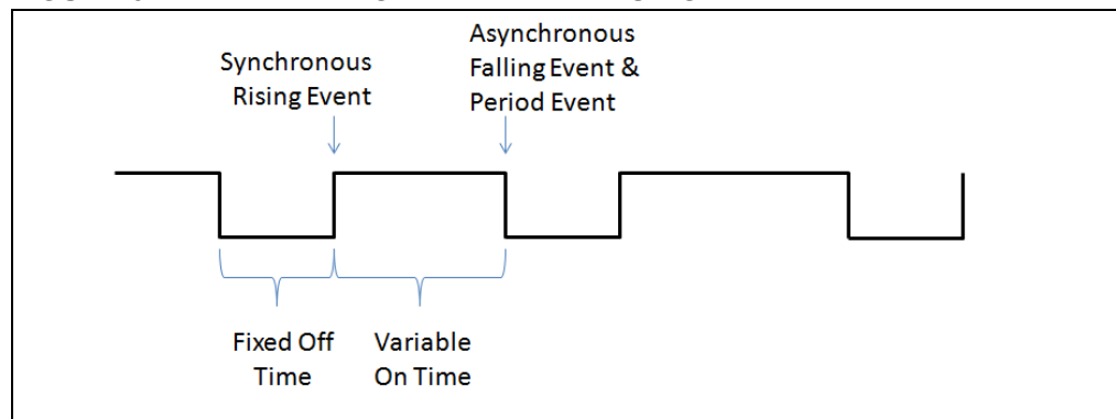
FIGURE 3-1: FIXED OFF-TIME WITH RISING EVENT DELAY
