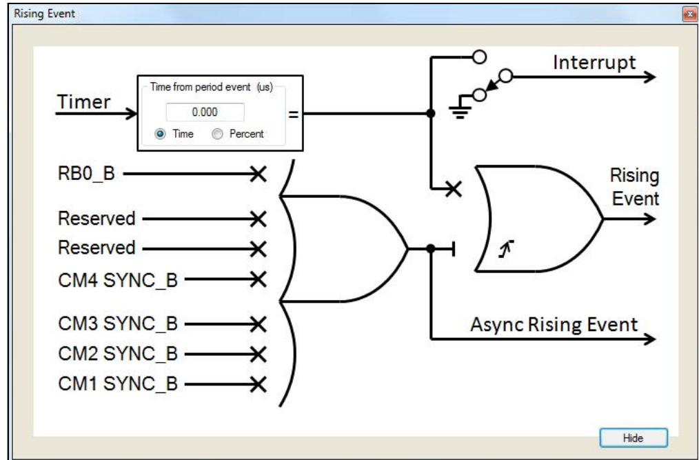
FIGURE 2-6: RISING EVENT CONTROL
