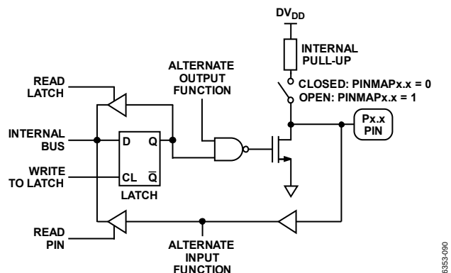
Figure 116. Port 0 Bit Latch and I/O Buffer
