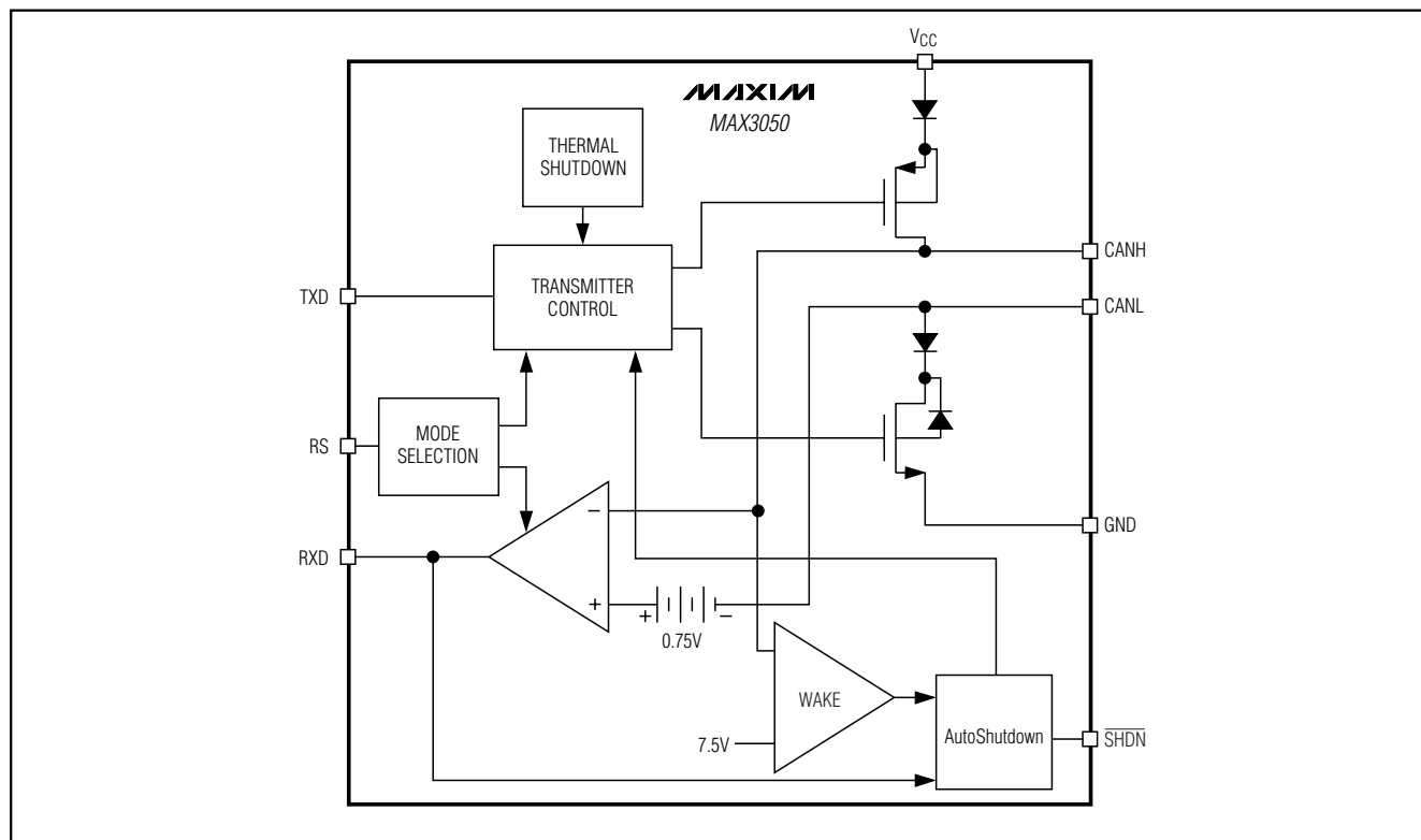
Figure 4. Functional Diagram
