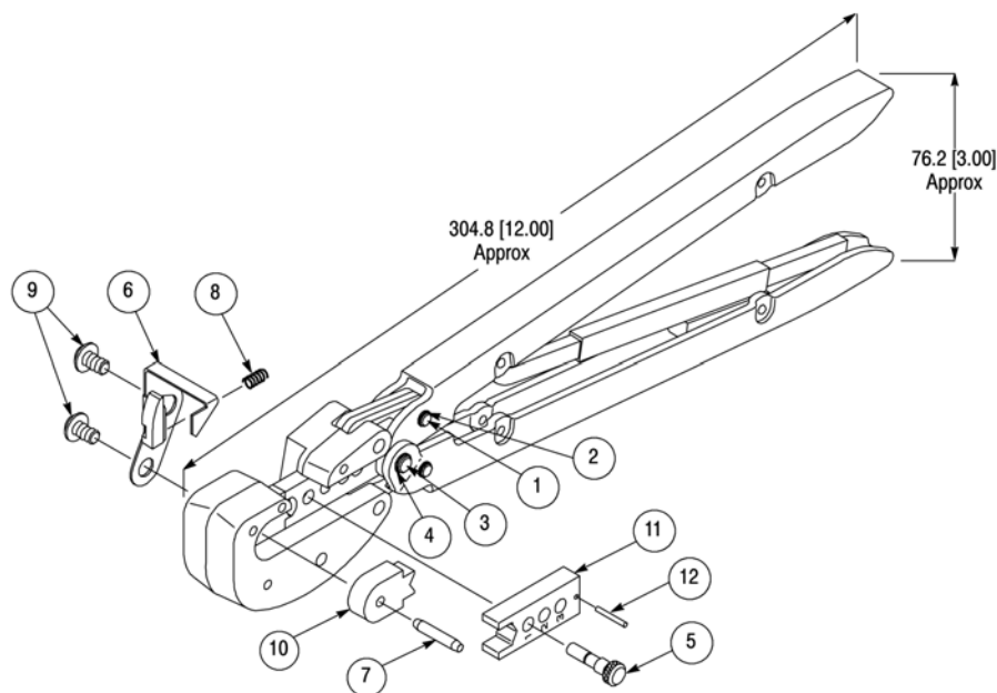
REPLACEMENT PARTS
