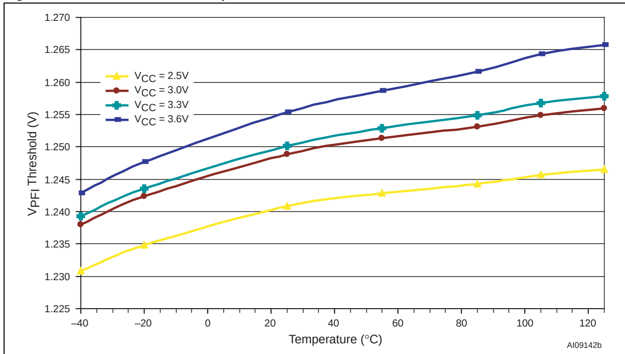
Figure 20. V PEI Threshold vs. Temperature
