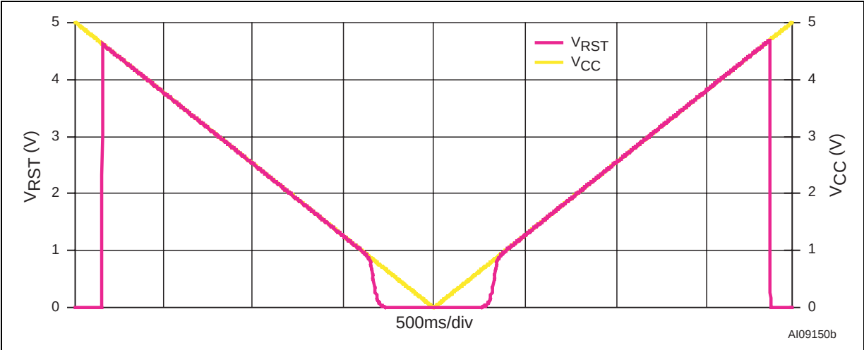
Figure 30. RST Output Voltage vs. Supply Voltage
