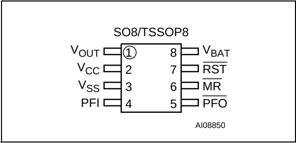
Figure 6. STM704/806 Connections
