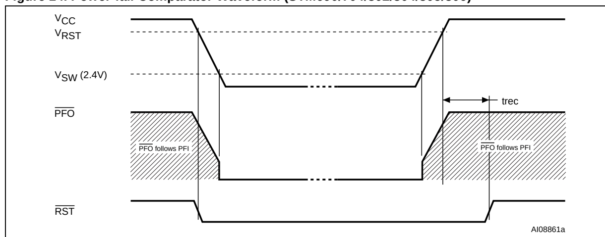
Figure 14. Power-fail Comparator Waveform (STM690/704/802/804/805/806)
