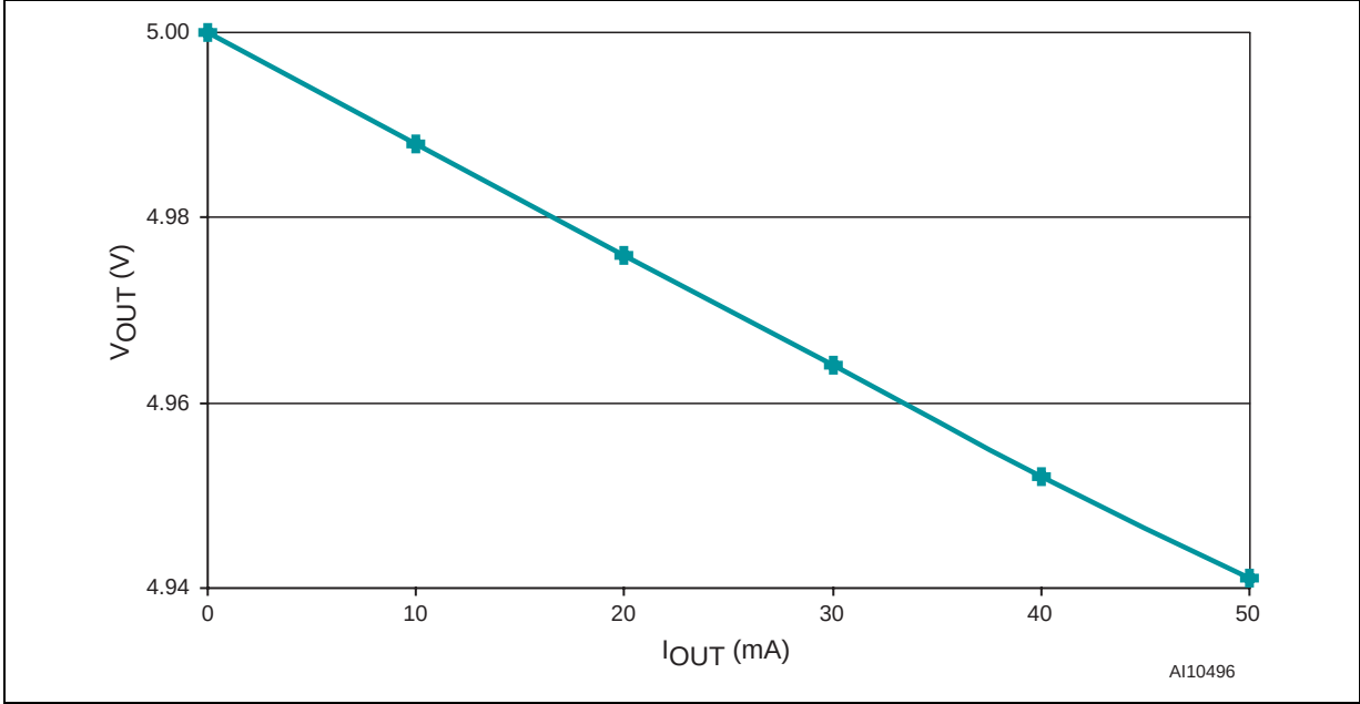
Figure 27. Output Voltage vs. Load Current ( V_{\text{CC}} = 5\text{V} ; V_{\text{BAT}} = 2.8\text{V} ; T_{\text{A}} = 25^{\circ}\text{C} )
