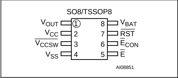
Figure 7. STM795 Connections
