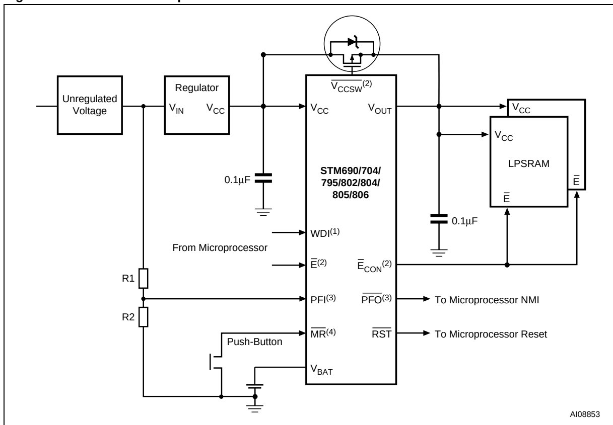
Figure 11. Hardware Hookup
