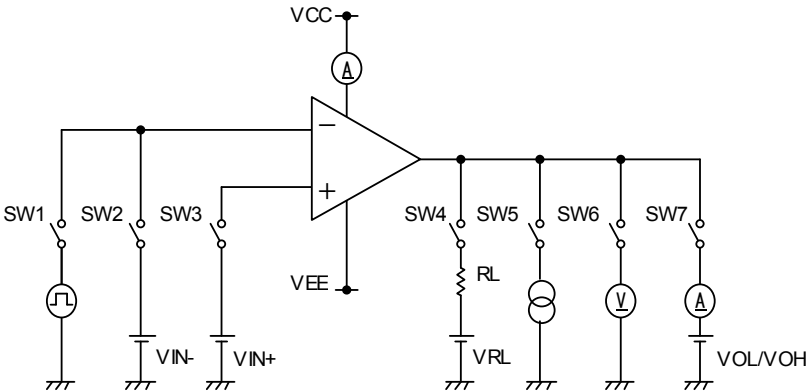
Fig.89 Measurement Circuit 2 (one channel only)
