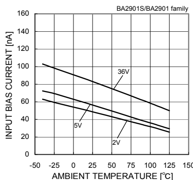
Fig. 74 Input Bias Current - Ambient Temperature
