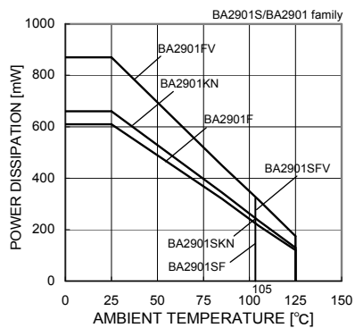
Fig. 64 Derating Curve
