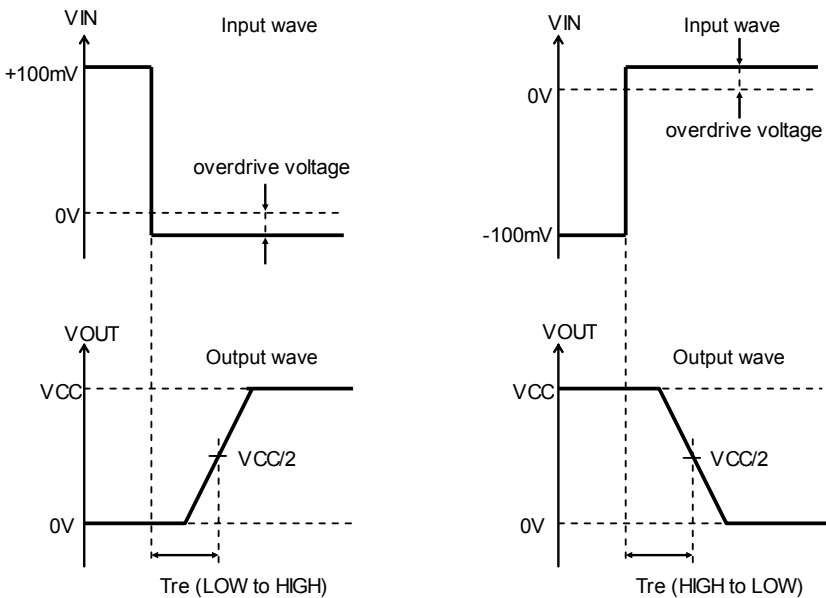
Fig.90 Response Time
