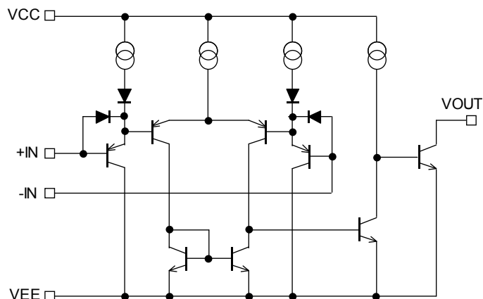
Fig.87 Circuit Diagram (one channel only )
