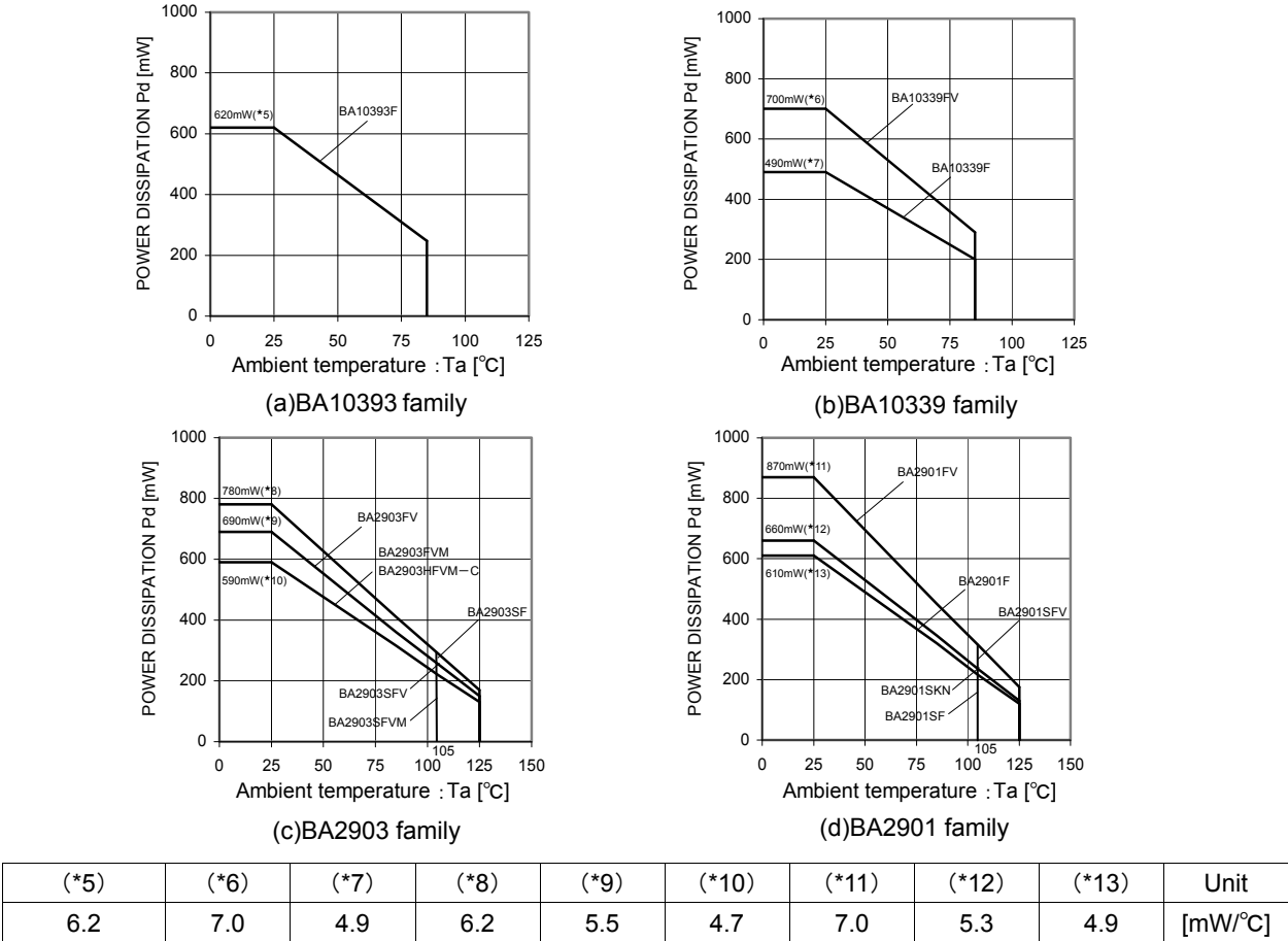
Fig.92 Derating curve
