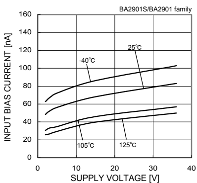
Fig. 73 Input Bias Current - Supply Voltage
