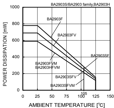
Fig. 41 Derating Curve
