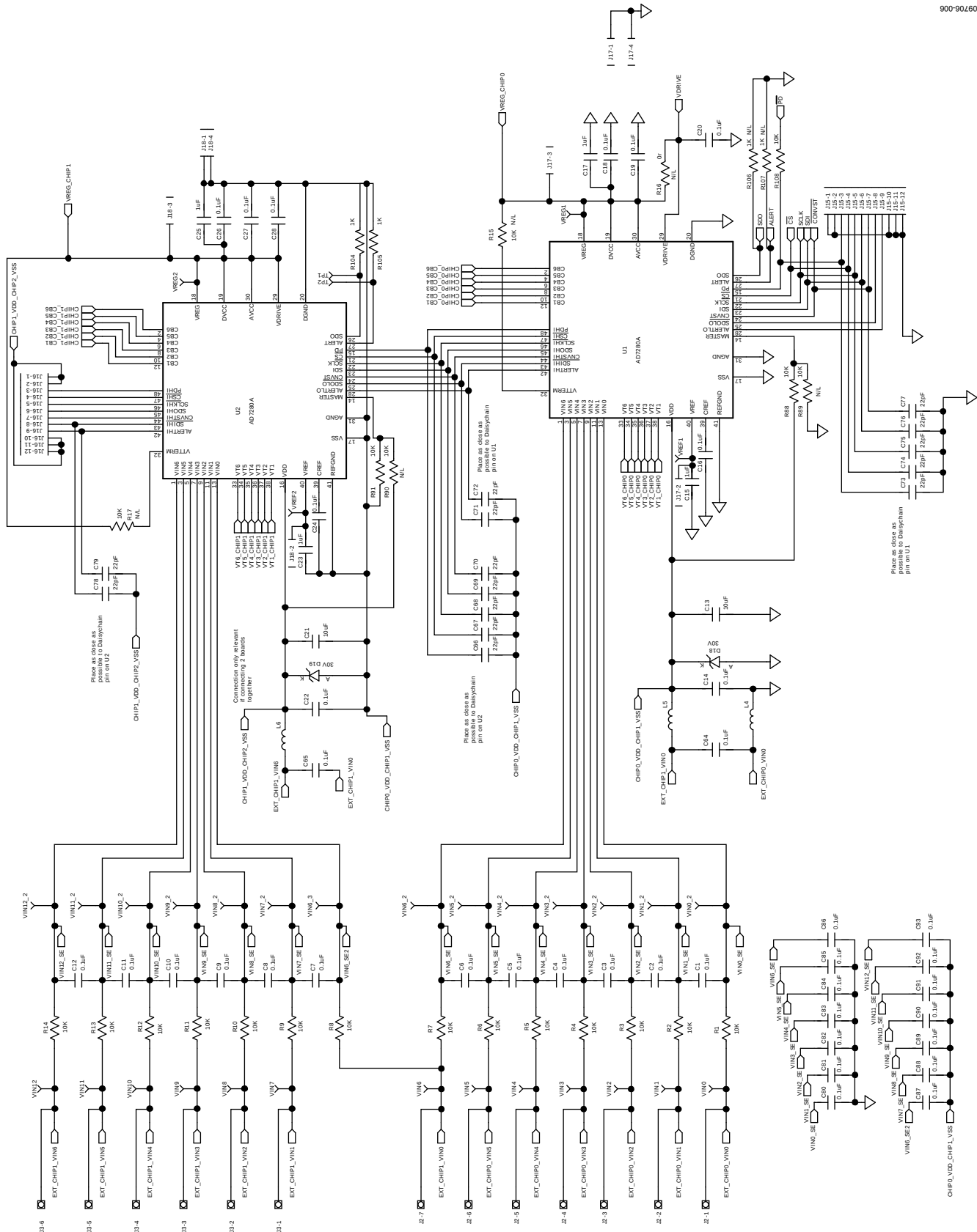
Figure 6. EVAL-AD7280AEDZ Schematic—Page 1
