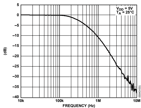
Figure 28. Multiplying Bandwidth
