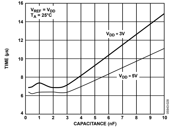
Figure 25. Settling Time vs. Capacitive Load
