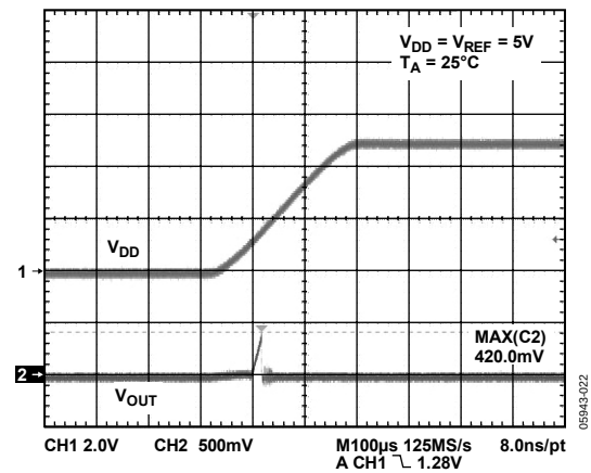
Figure 20. Power-On Reset to 0\text{ V}
