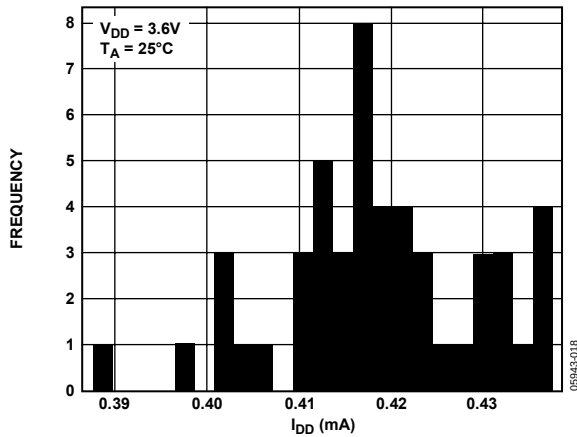
Figure 16. I_{DD} Histogram with V_{DD} = 3.6\text{ V}
