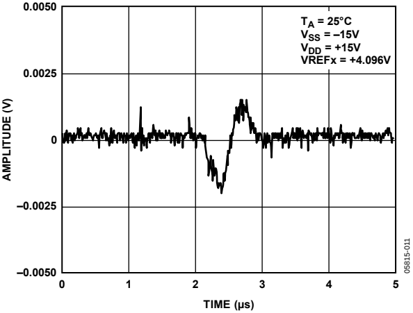
Figure 12. Digital Crosstalk
