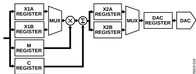
Figure 19. Data Registers Associated with Each DAC Channel
