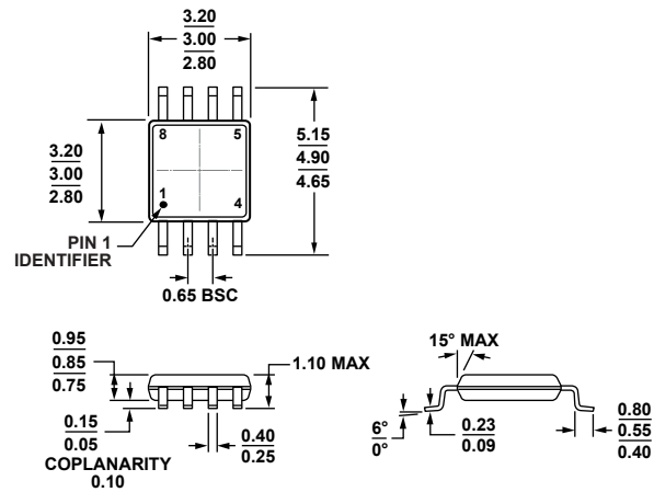
Figure 66. 8-Lead Mini Small Outline Package [MSOP] (RM-8) Dimensions shown in millimeters
