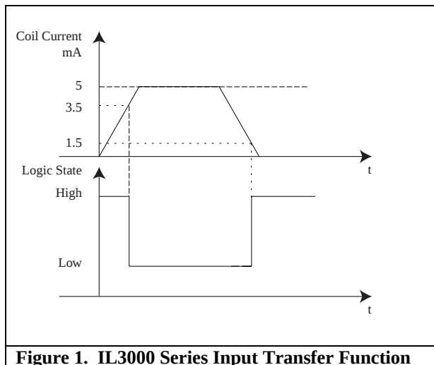
Figure 1. IL3000 Series Input Transfer Function
