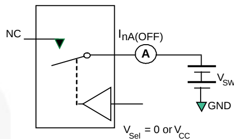
Figure 10. Off Leakage
