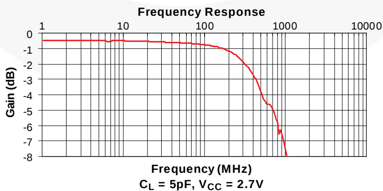
Figure 8. Bandwidth
