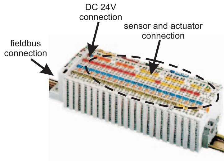
Fig. 4-1. Connection Example and Principle of a Fieldbus Node for a Network Architecture 1Netzwerkknötene
