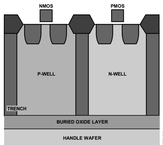
Figure 36. Trench Isolation
