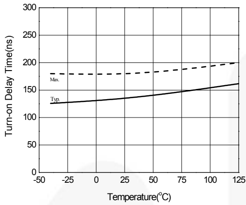
Figure 4. Turn-on Propagation Delay vs. Temperature
