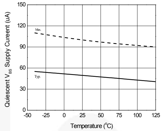
Figure 11. Quiescent V_{BS} Supply Current vs. Temperature
