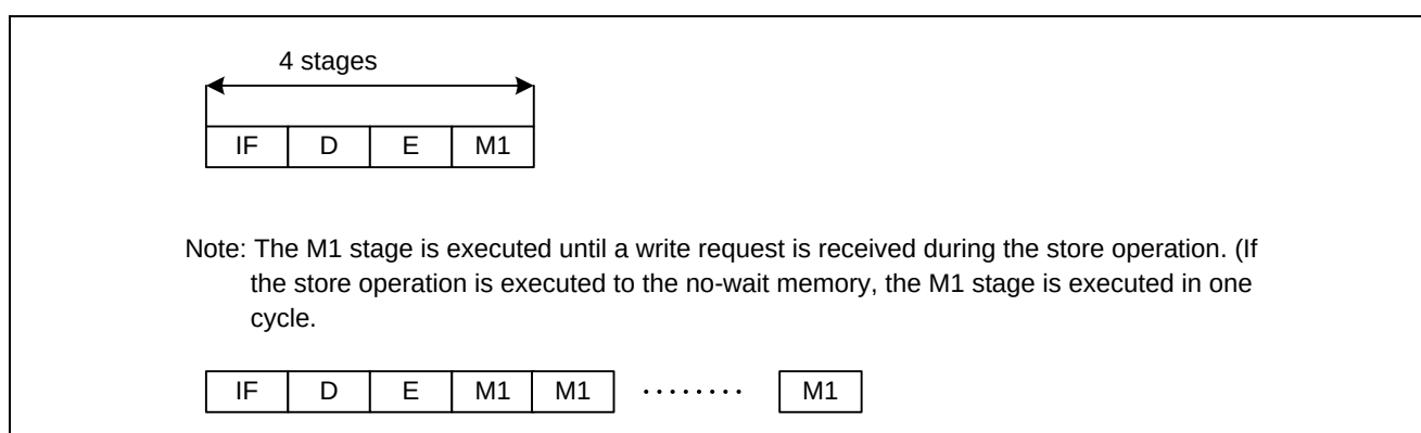
Figure 2.13 Store Operation
