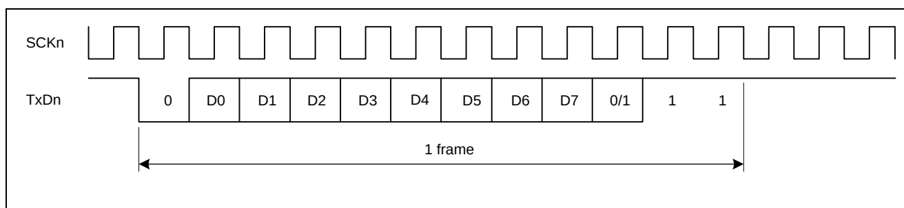
Figure 20.6 Phase Relationship between Output Clock and Transmit Data (Asynchronous Mode)
