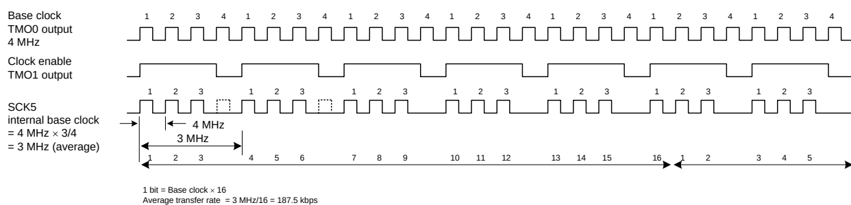
Figure 20.3 Example of Average Transfer Rate Setting when TMR Clock is Input
