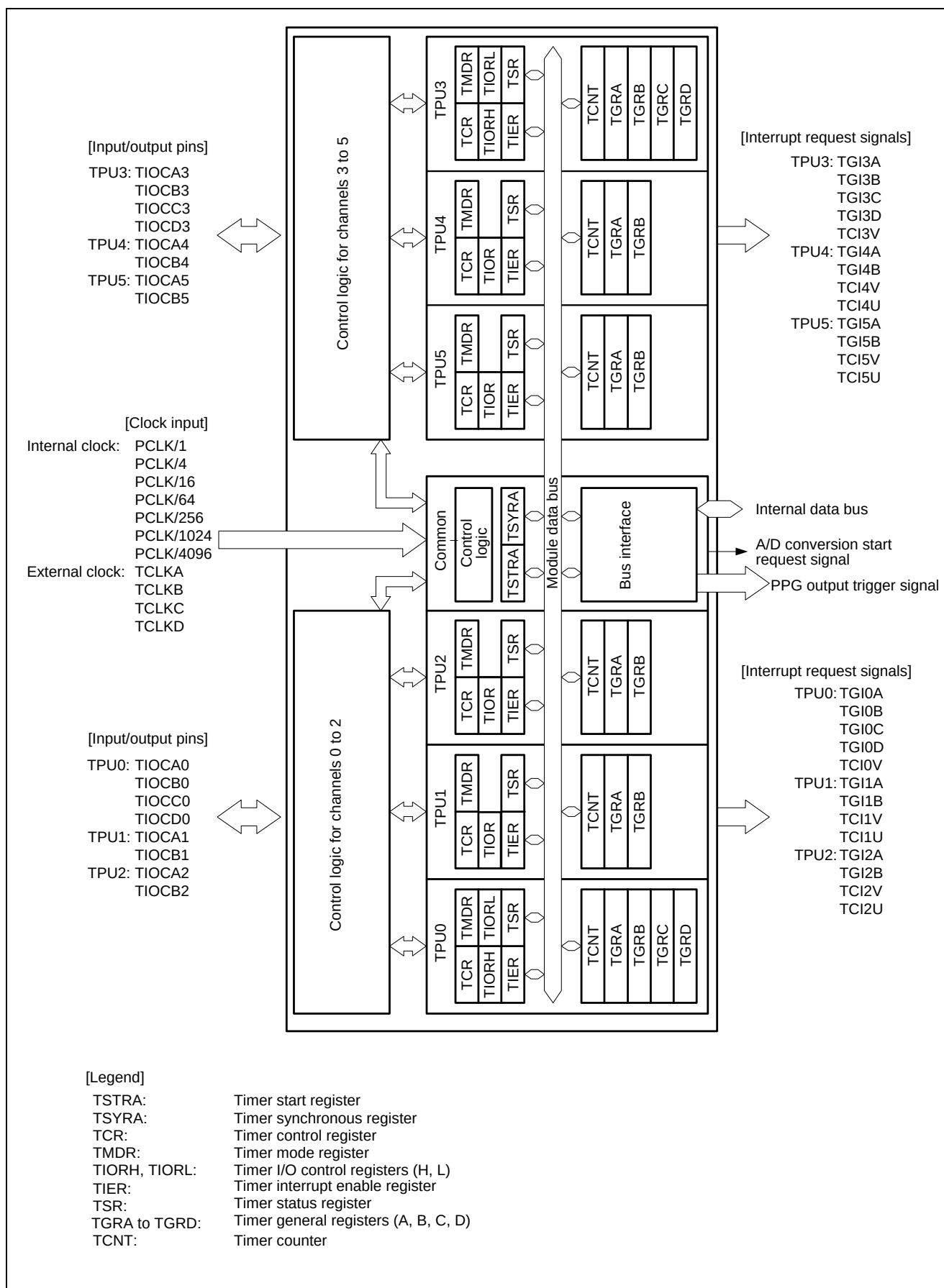
Figure 15.1 Block Diagram of TPU (Unit 0)
