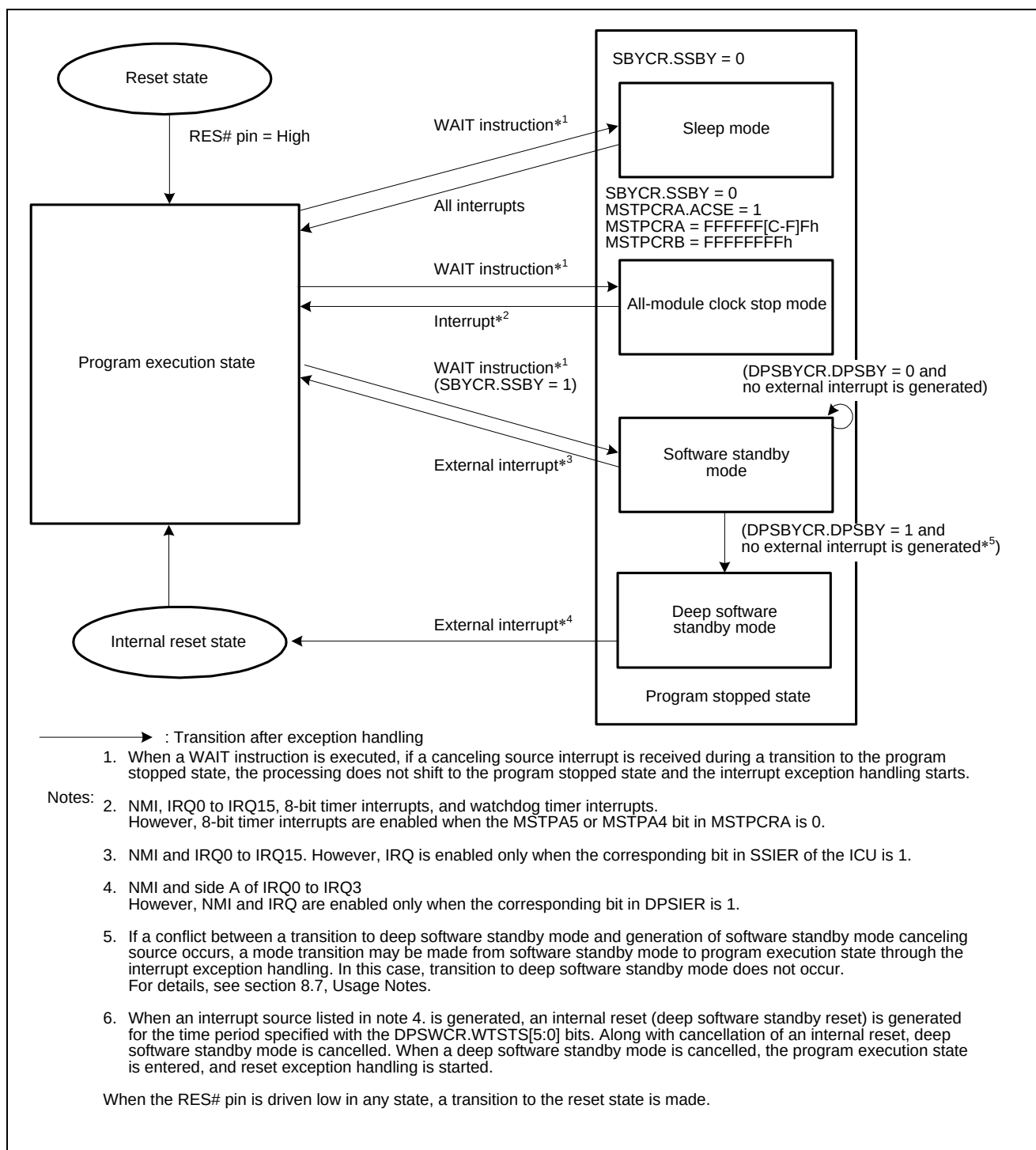
Figure 8.1 Mode Transitions
