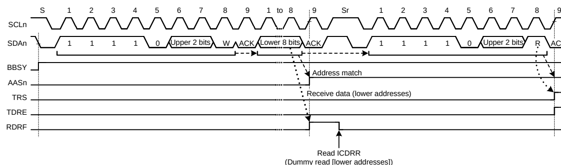
Figure 22.24 Timing of AASy Flag Setting to 1 with 10-Bit Address Format Selected
