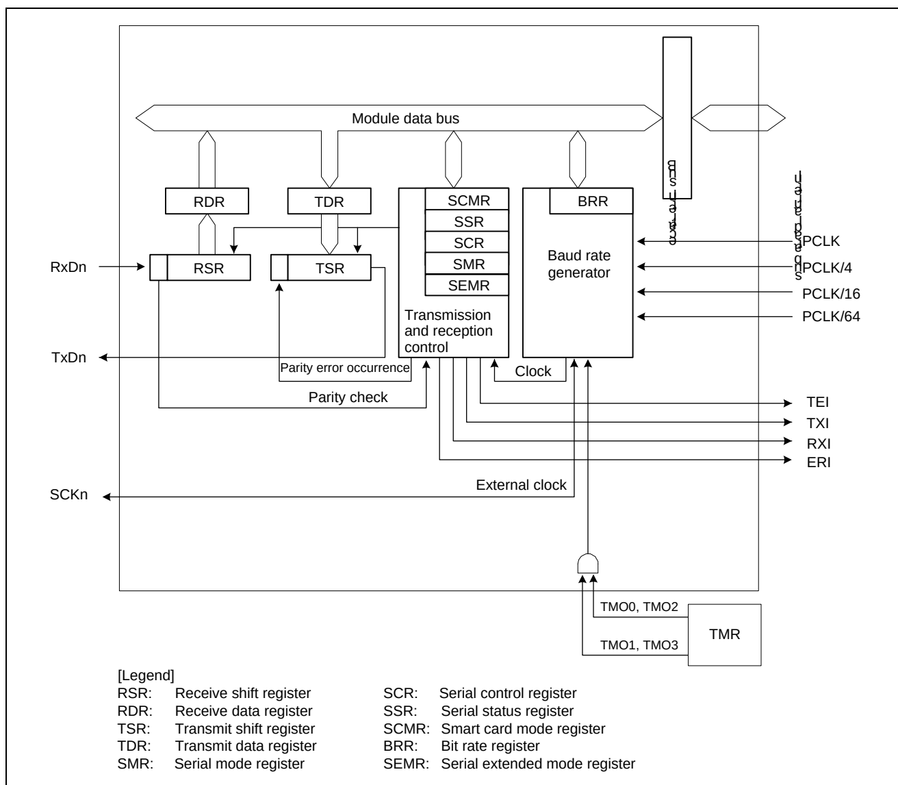
Figure 20.2 Block Diagram of SCI5 and SCI6
