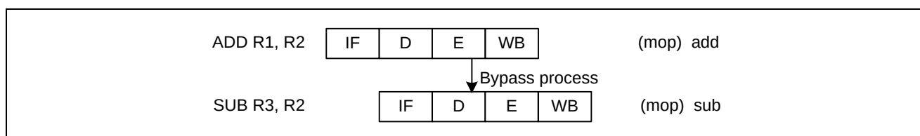
Figure 2.24 Bypass Process
