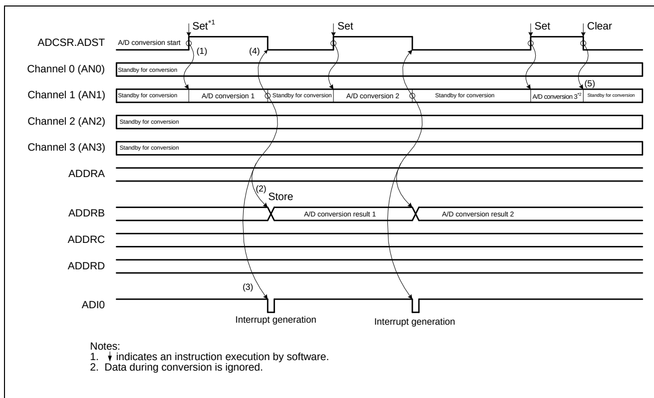
Figure 23.5 Example of A/D Converter Operation (Single Mode)
