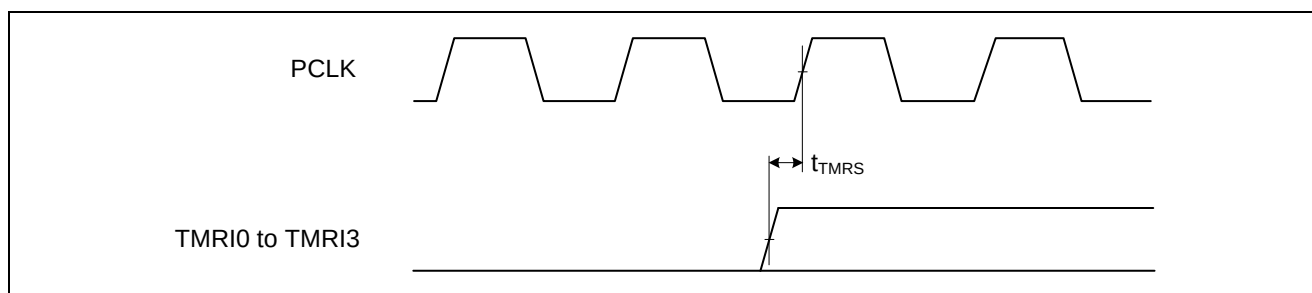
Figure 29.19 8-Bit Timer Reset Input Timing
