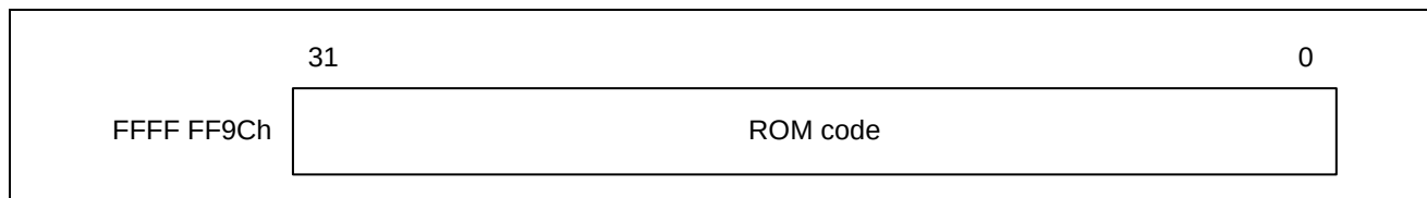
Figure 26.33 Configuration of a ROM Code
