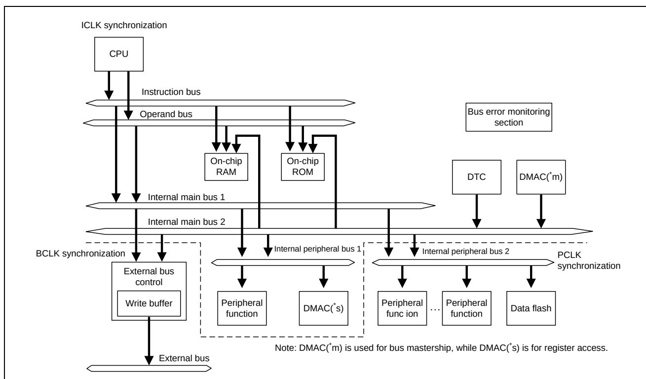
Figure 11.1 Bus Configuration
