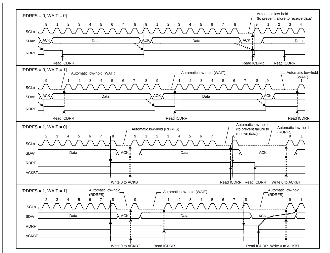
Figure 22.31 Automatic Low-Hold Operation in Receive Mode (Using RDRFS and WAIT Bits)
