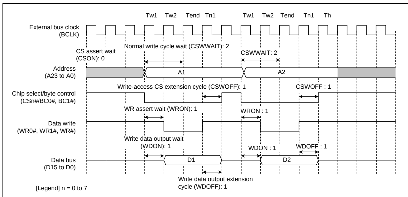
Figure 11.11 Example of Normal-Write Operation (when Two Rounds of Bus Access are Generated in Response to a Single Request for Transfer)
