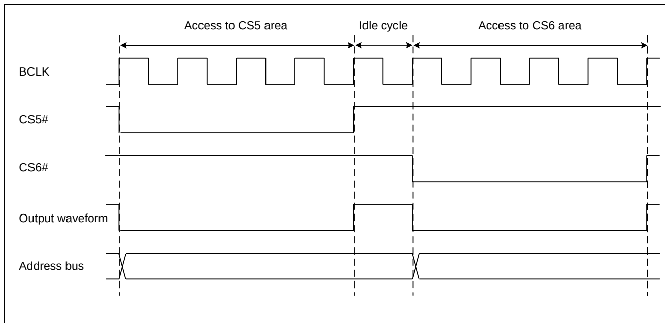
Figure 14.1 Timing for Output of CSn# Signals to the Same Pin
