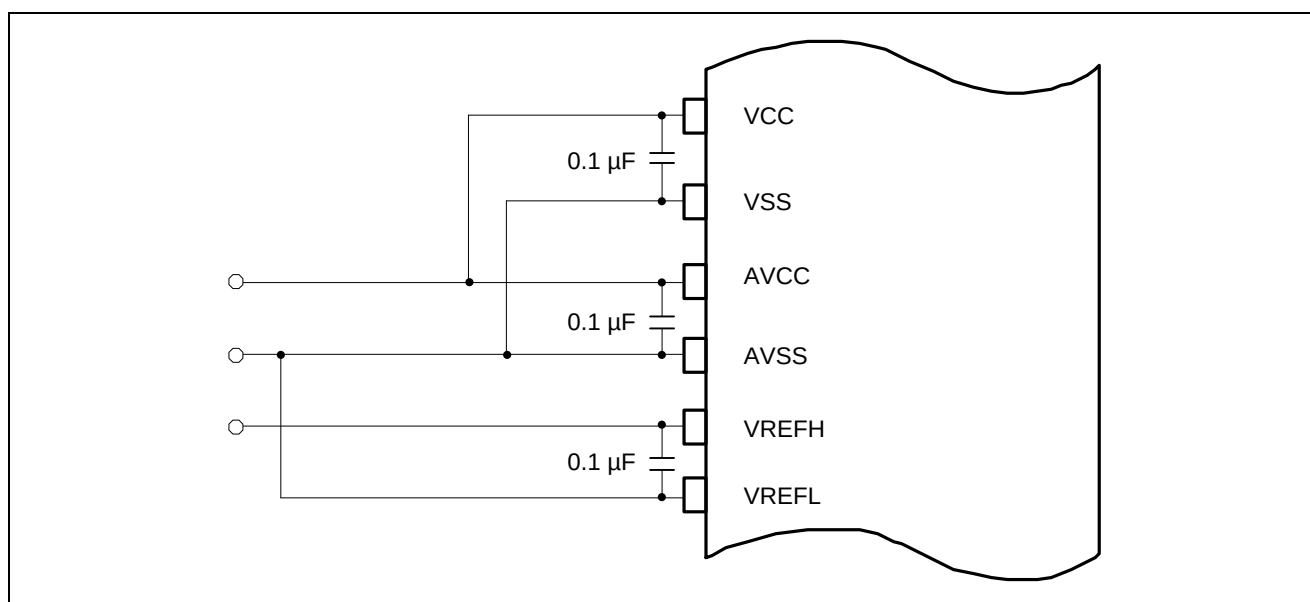
Figure 23.16 Example of Connection for Power-Supply Pins
