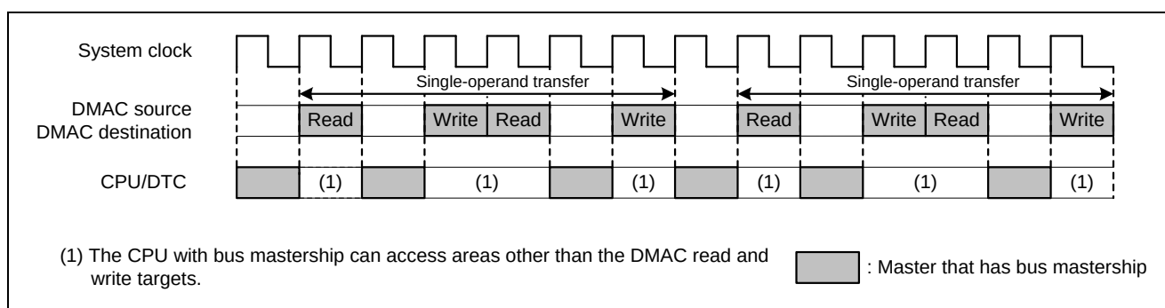
Figure 12.2 Example of how Bus Mastership Passes between the DMAC and Other Bus Masters
