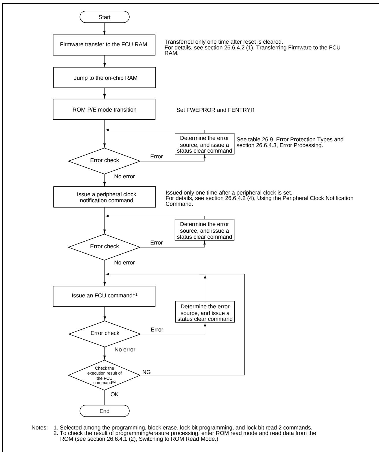
Figure 26.11 Simple Flowchart of the Procedure for Programming and Erasure
