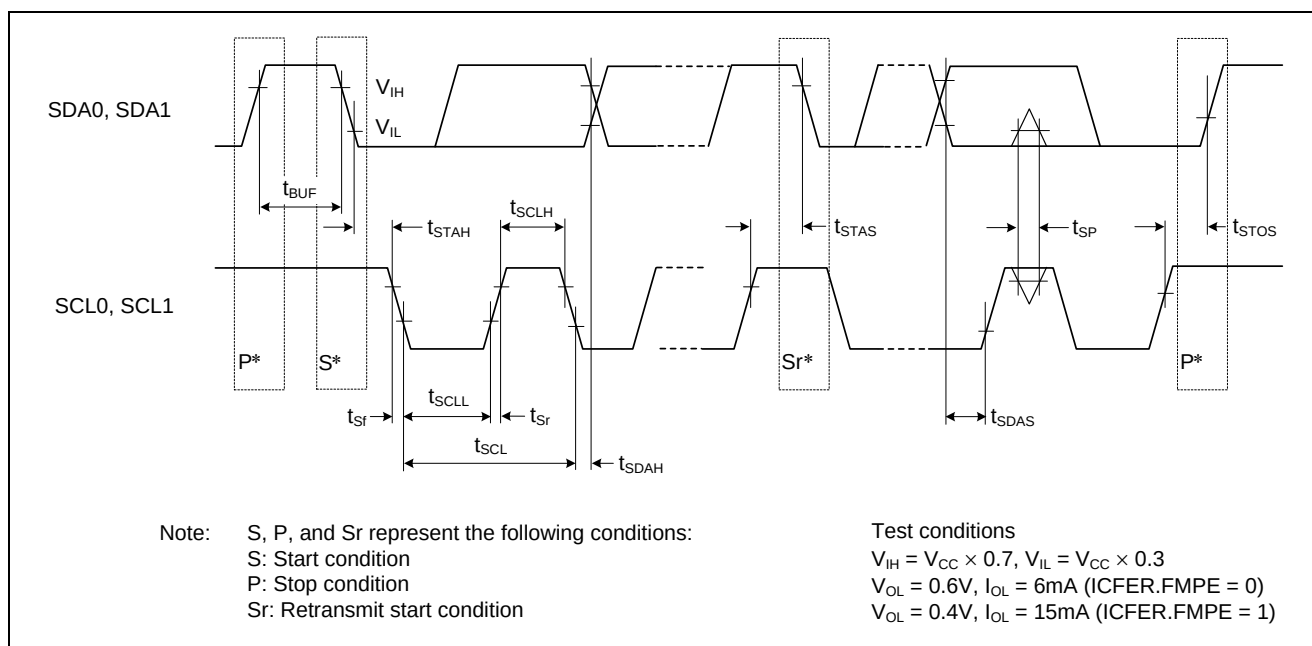
Figure 29.25 I²C Bus Interface Input/Output Timing
