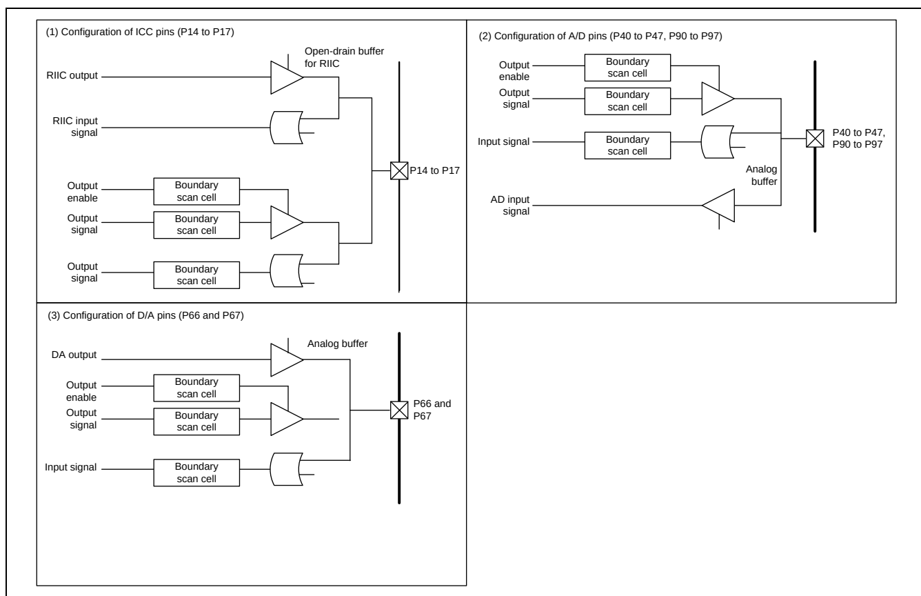
Figure 28.4 Pin Configuration
