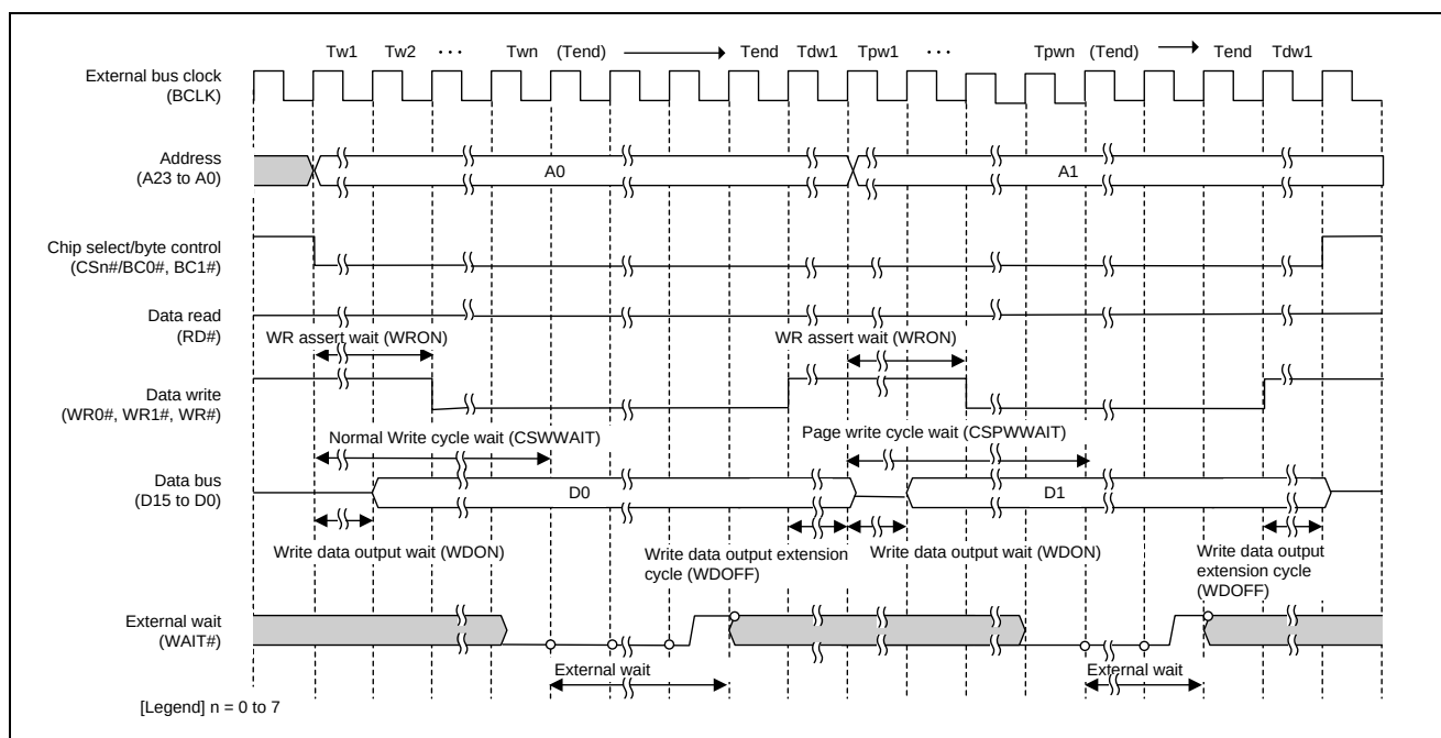
Figure 11.20 Example of External Wait Timing (Page-Write Access to 16-Bit Bus Space)
