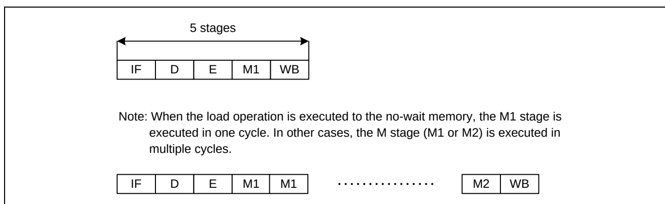
Figure 2.12 Load Operation
