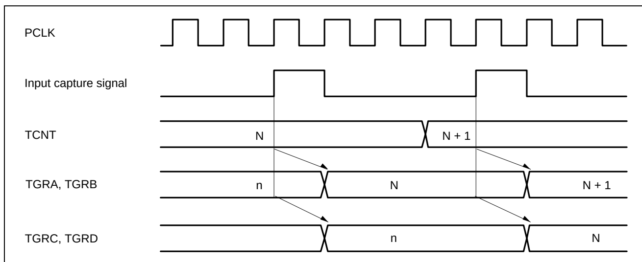
Figure 15.38 Buffer Operation Timing (Input Capture)
