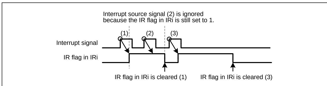
Figure 10.3 Timing for Re-setting the IR Flag in IRI
