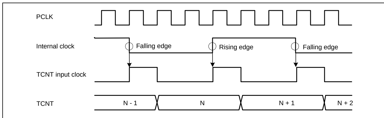
Figure 15.31 Count Timing in Internal Clock Operation
