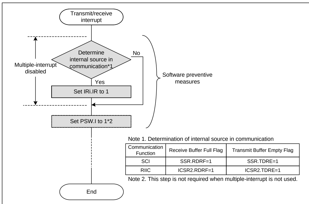
Figure 10.10 Flowchart for Measures with DISEL = 1
