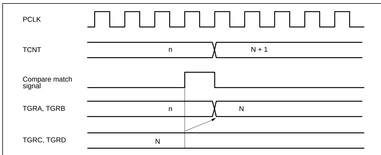
Figure 15.37 Buffer Operation Timing (Compare Match)
