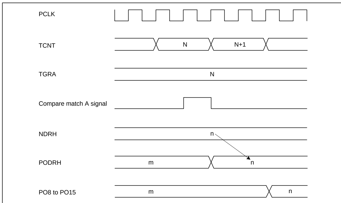
Figure 16.5 Timing of Transfer and Output of the Values in NDR (Example)
