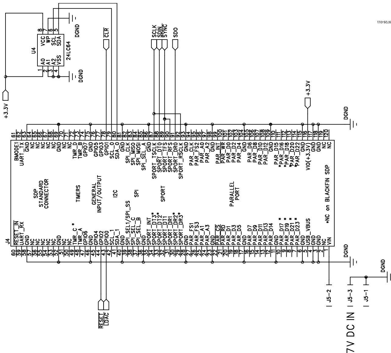
Figure 11. Schematic of the SDP Board Connector
