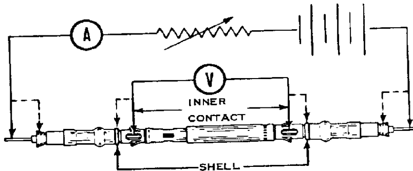
FIGURE I CONTACT RESISTANCE
