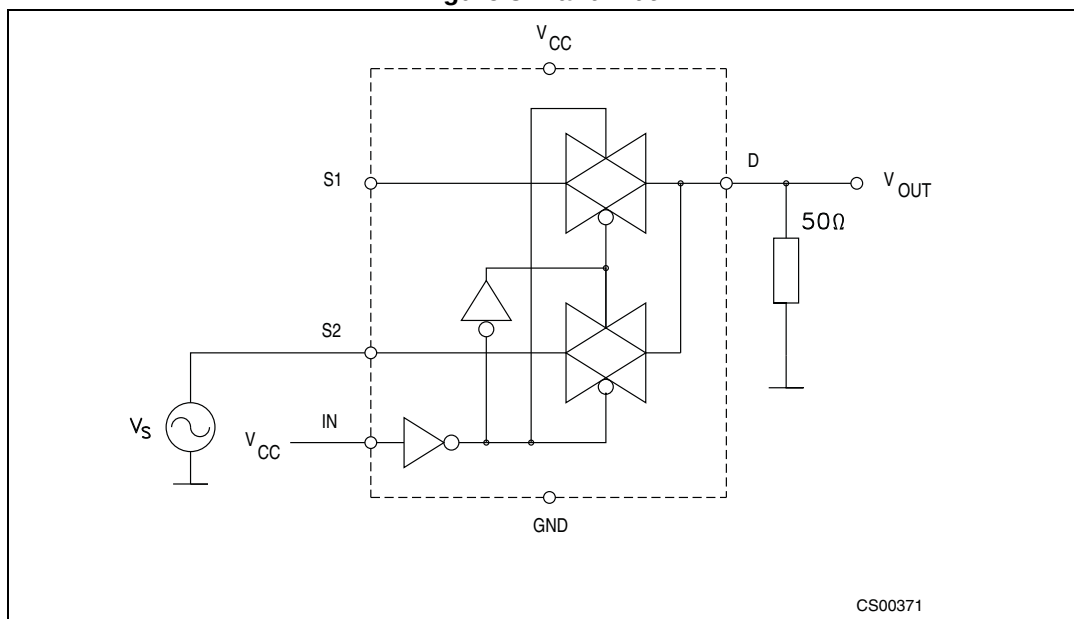
Figure 9. Channel-to-channel crosstalk
