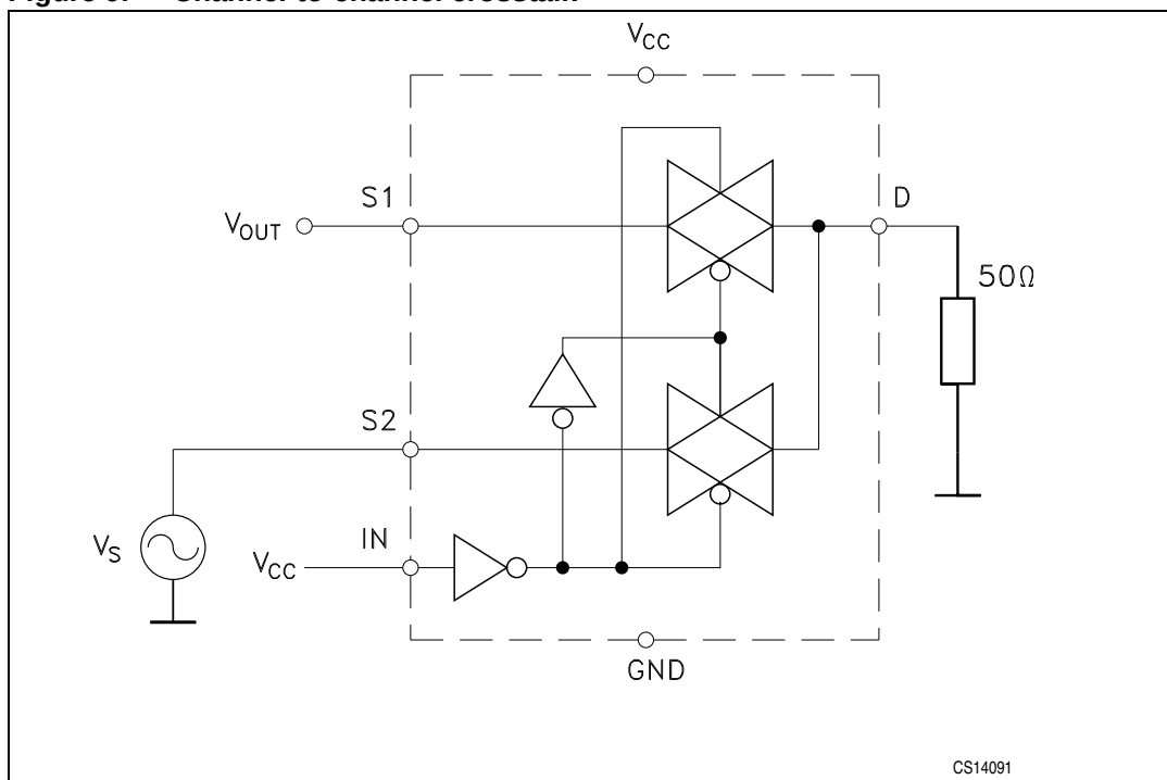
Figure 9. Channel-to-channel crosstalk
