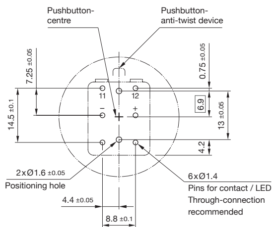
Component layout 5
