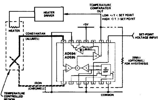
Figure 9. Set-Point Controller
