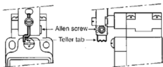
Figure 13. Allen Screw and Teller Tab Location
