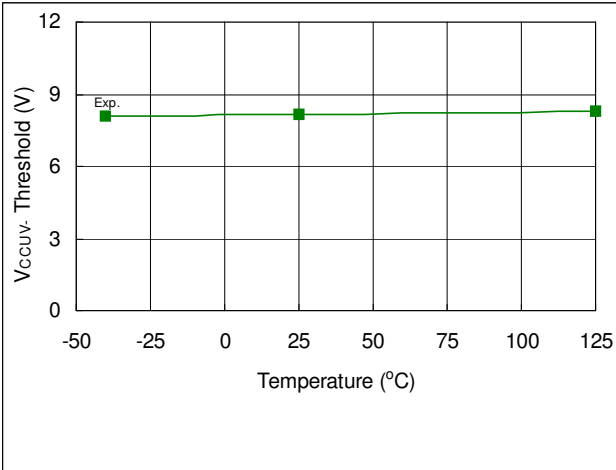
Fig. 33. V CCUV- Threshold vs. Temperature
