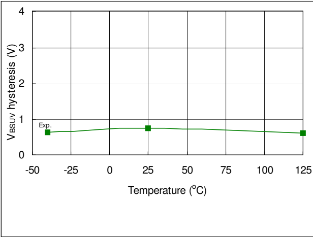
Fig. 29. V BS Supply UV Hysteresis vs. Temperature
