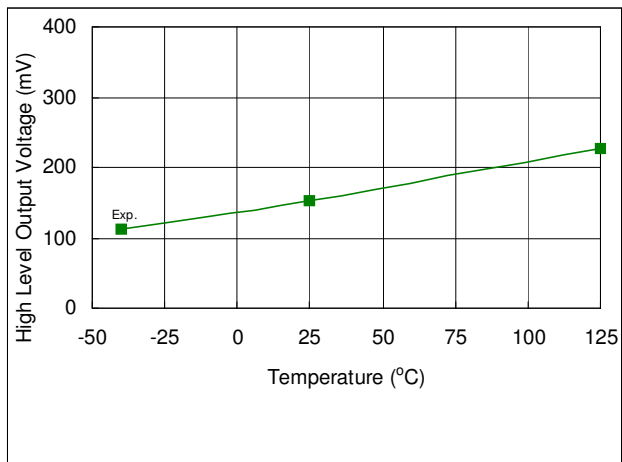
Fig. 37. High Level Output Voltage vs. Temperature
