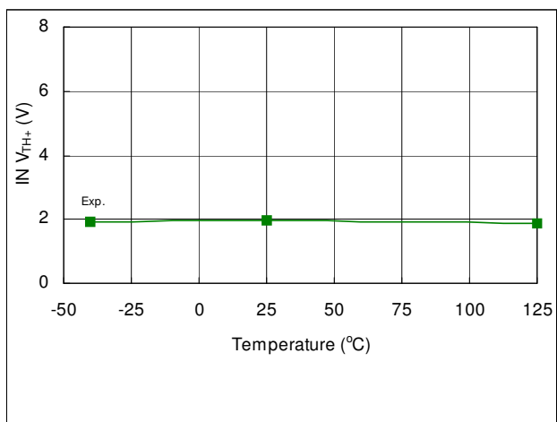
Fig. 39. IN V_{TH+} vs. Temperature
