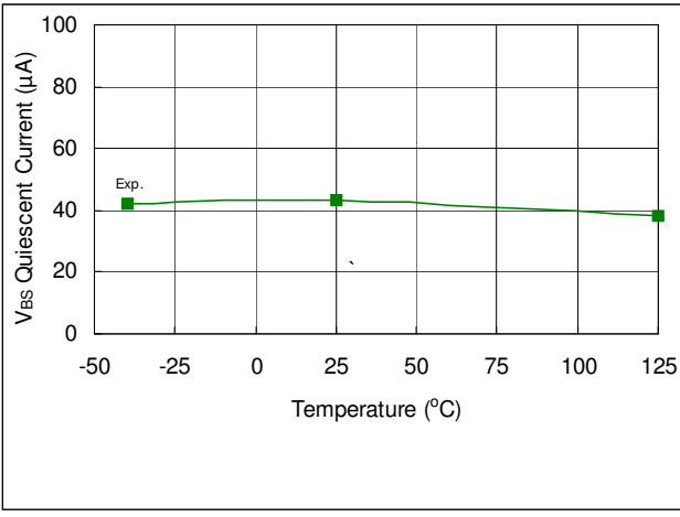
Fig. 31. V BS Quiescent Supply Current vs. Temperature
