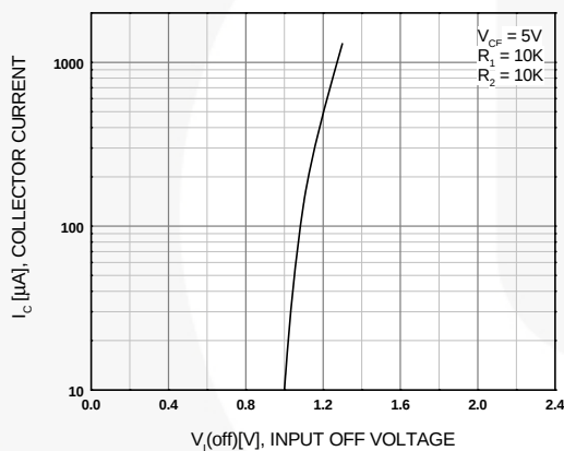
Figure 3. Input-Off Voltage
