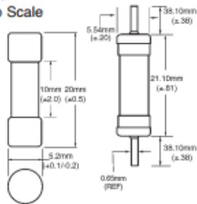
Dimensions - mm Drawing Not to Scale
