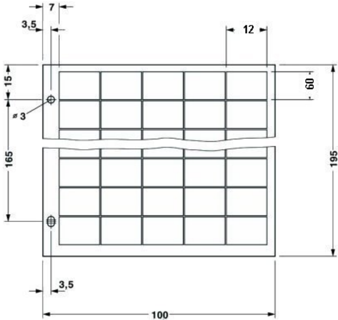
Dimensioned drawing
