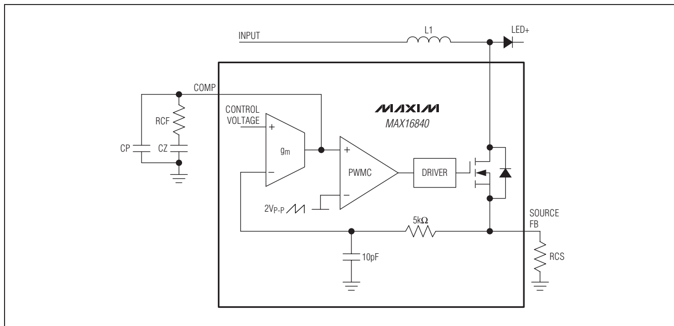
Figure 1. Control Loop
