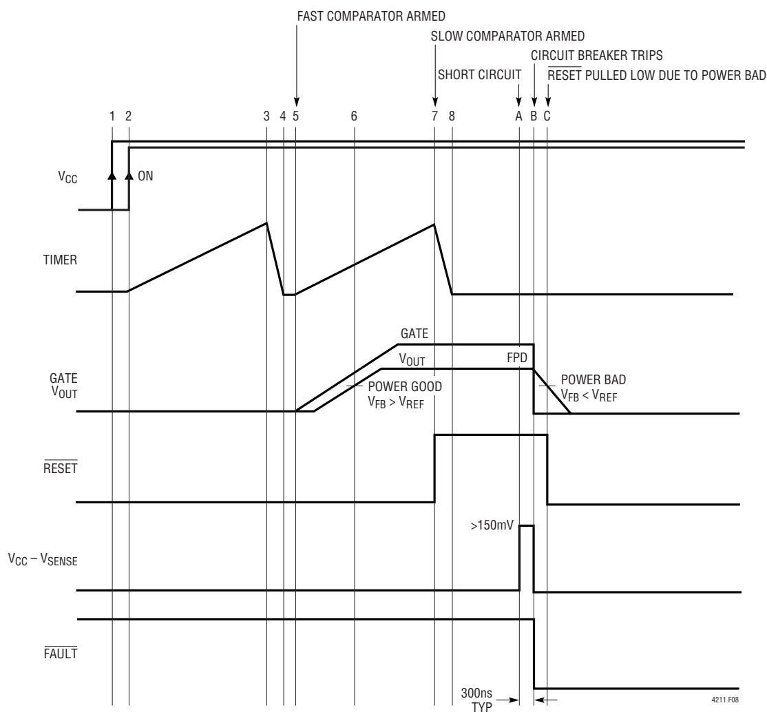
Figure 8. Output Short Circuit Causes Fast Comparator to Trip the Circuit Breaker
