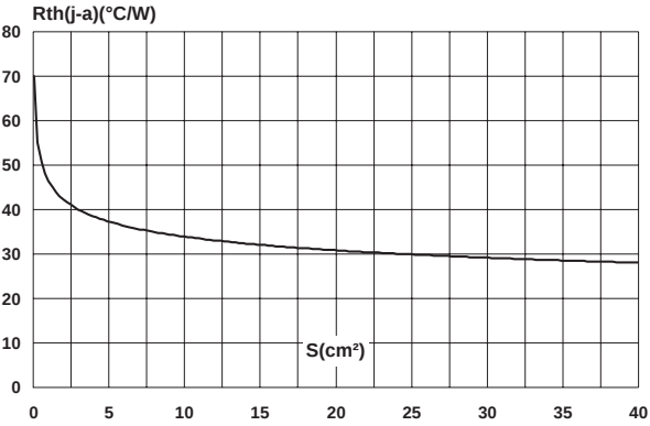
Fig. 10: Thermal resistance junction to ambient versus copper surface under tab (epoxy printed board FR4, Cu = 35μm).(STPS41H100CG only)
