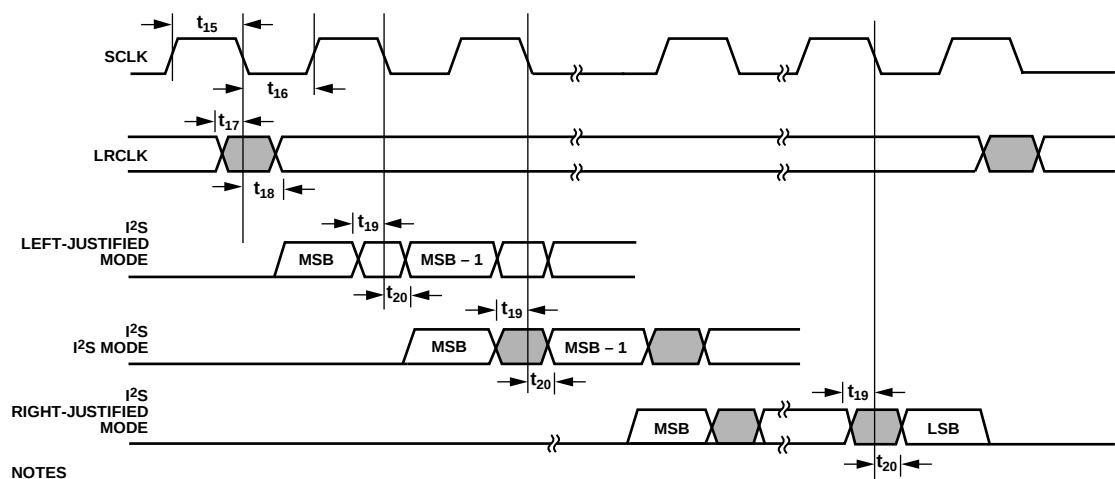
Figure 5. I²S Timing
