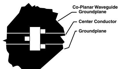
Figure 17. Circuit Layout.
