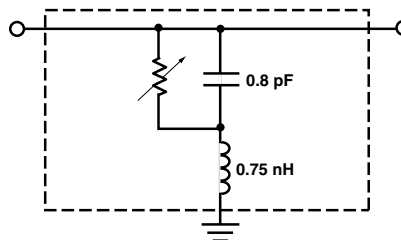
Figure 17. Circuit Layout.
