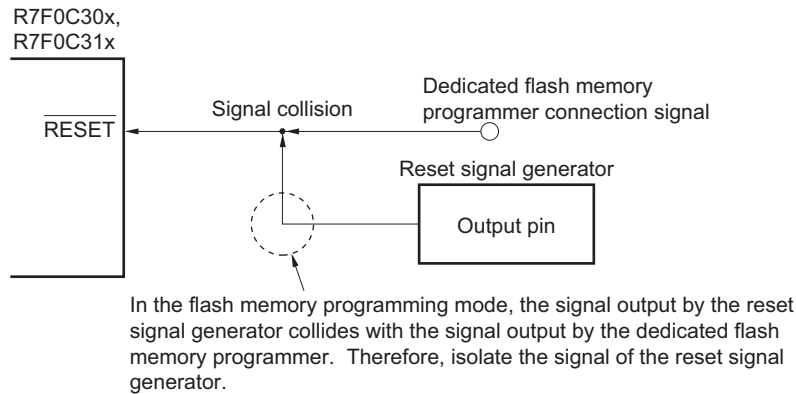
Figure 21-4. Signal Collision ( \overline{\text{RESET}} Pin)
