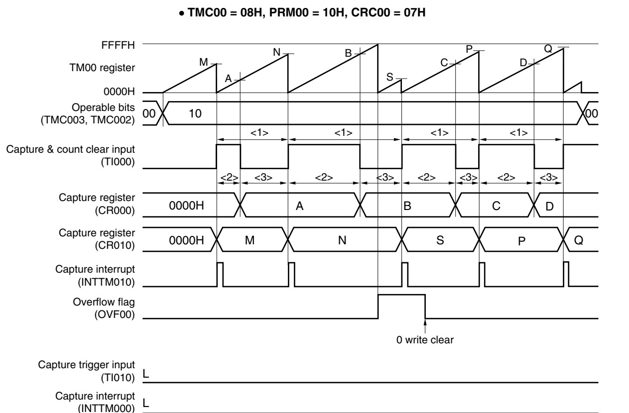
Figure 6-51. Timing Example of Pulse Width Measurement (3)
