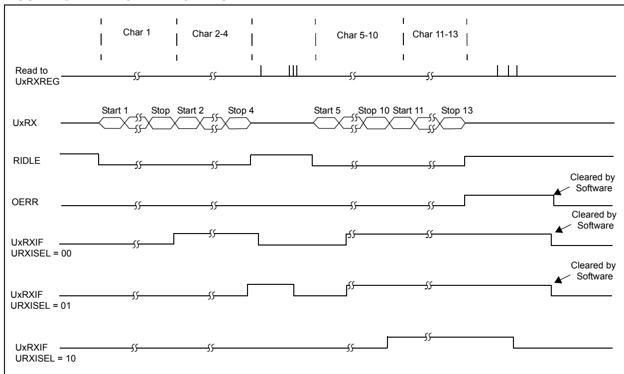
FIGURE 19-2: UART RECEPTION
