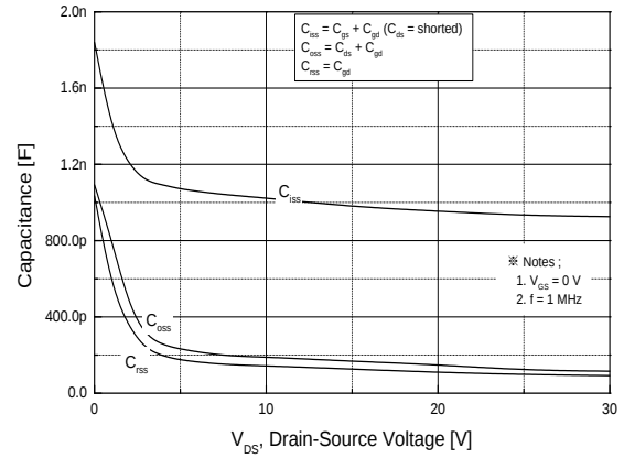
Fig.8 Capacitance Characteristics
