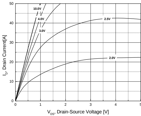
Fig.1 On-Region Characteristics
