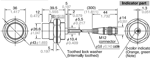
GX-30MLU GX-30MLUB Sensor
