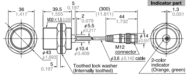
GX-30MU-J GX-30MUB-J GX-F30MU-J Sensor
