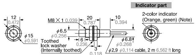
GX-8MLU GX-8MLUB Sensor
