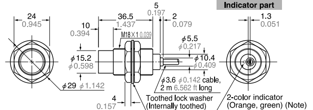
GX-18MLU GX-18MLUB Sensor
