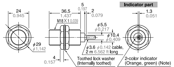
GX-18MU GX-18MUB Sensor
