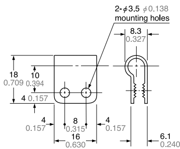
MS-SS5 Sensor mounting bracket for GX-5SU(B) (Optional)
