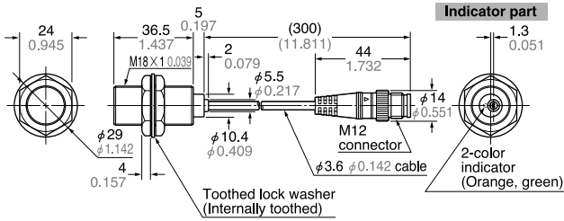
GX-18MU-J GX-18MUB-J GX-F18MU-J Sensor
