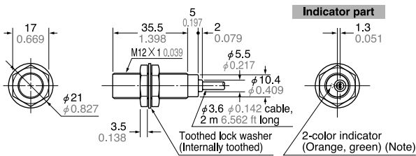
GX-12MU GX-12MUB Sensor
