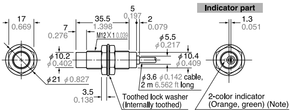
GX-12MLU GX-12MLUB Sensor
