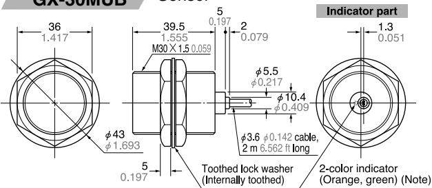
GX-30MU GX-30MUB Sensor
