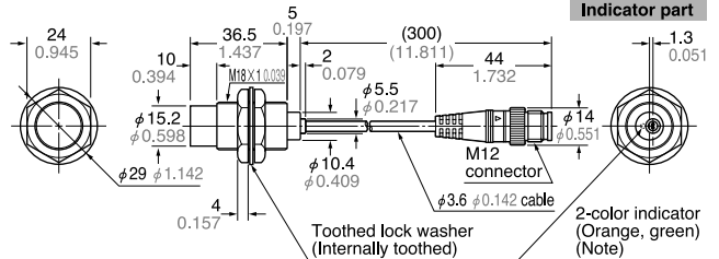
GX-18MLU-J GX-18MLUB-J Sensor
