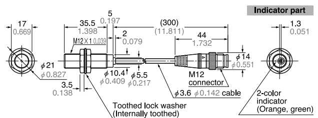
GX-12MU-J GX-12MUB-J GX-F12MU-J Sensor
