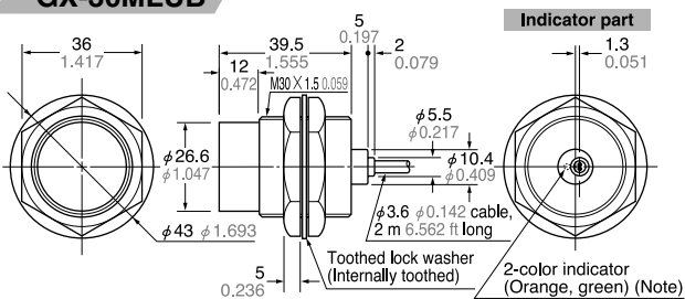
GX-30MLU GX-30MLUB Sensor
