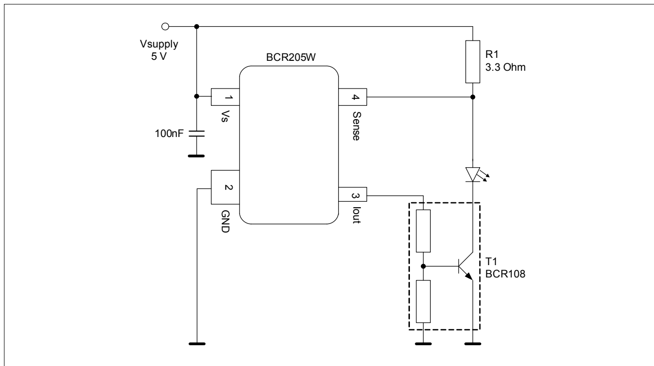
Figure 4 30 mA Application using BCR108
