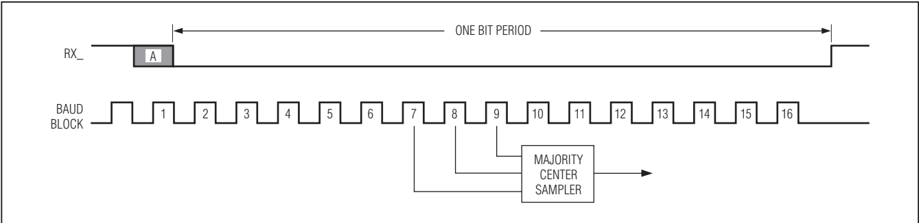
Figure 6. Midbit Sampling
