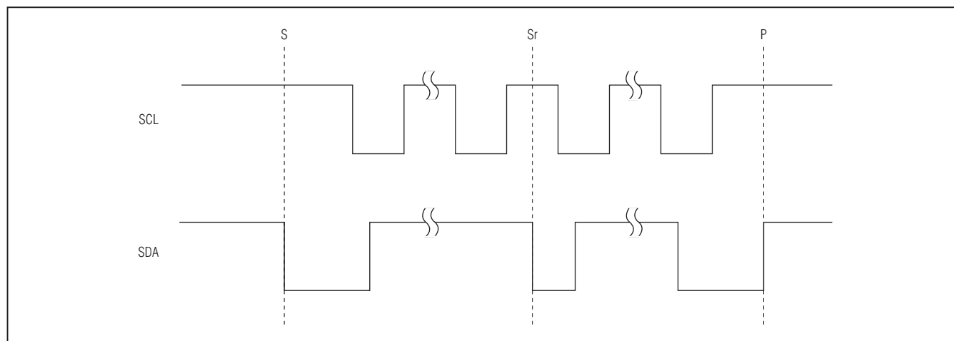
Figure 21. I²C START, STOP, and Repeated START Conditions
