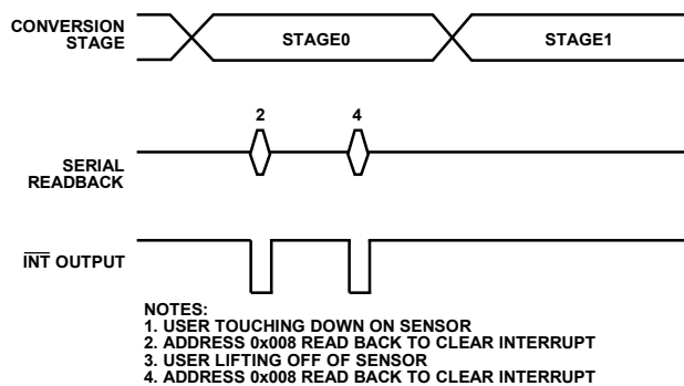
Figure 36. Example of Sensor Touch Interrupt
