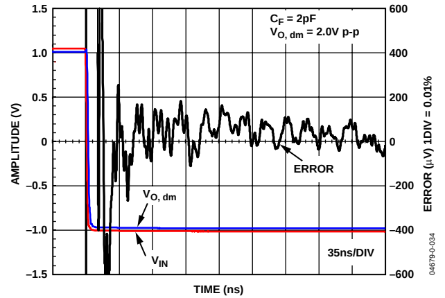
Figure 36. Settling Time (0.01%)
