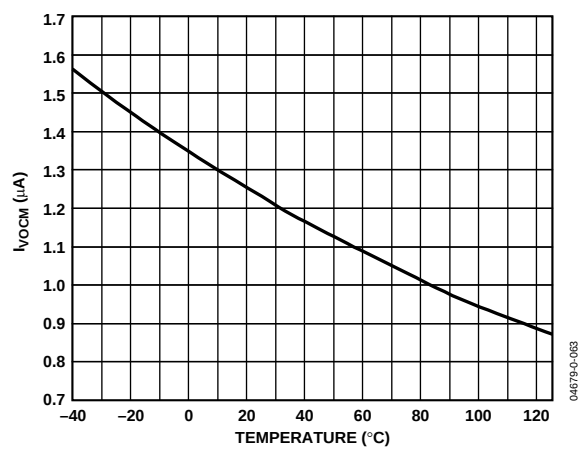
Figure 55. V_{OCM} Bias Current vs. Temperature
