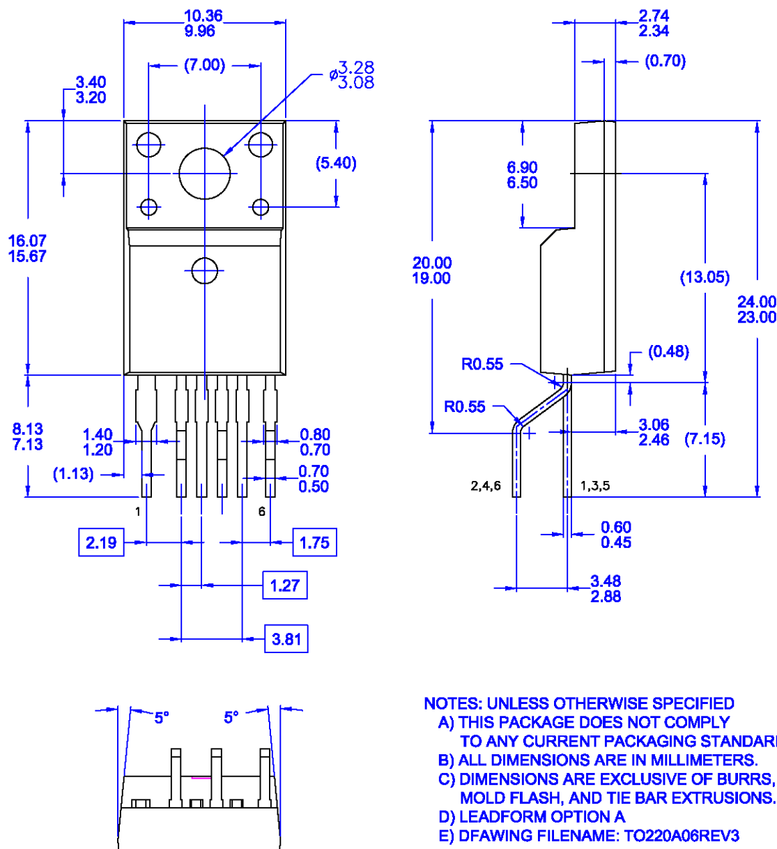
Figure 39. 6-Lead, TO-220 Package (Forming)
