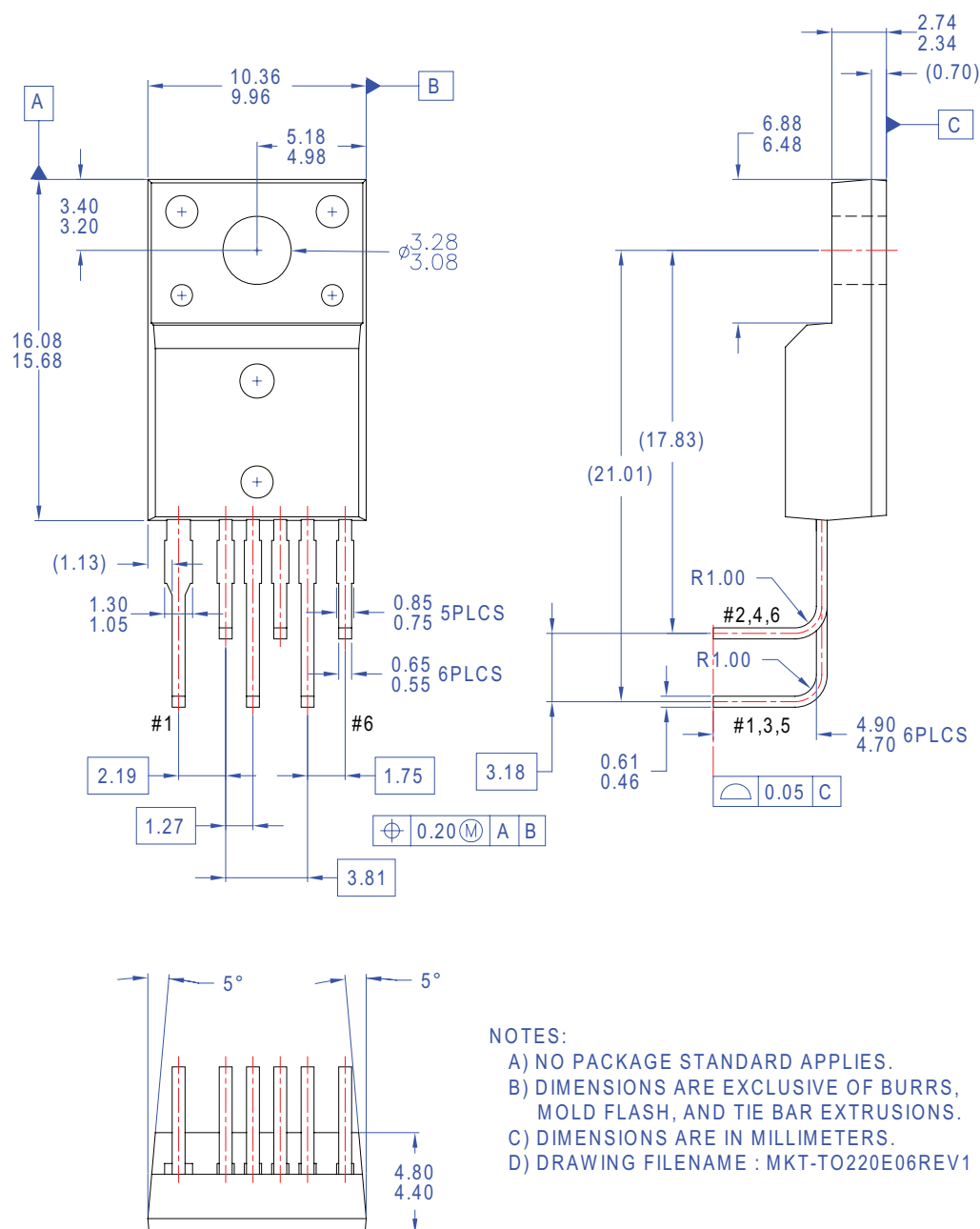
Figure 40. 6-Lead, TO-220 Package (L-Forming)
