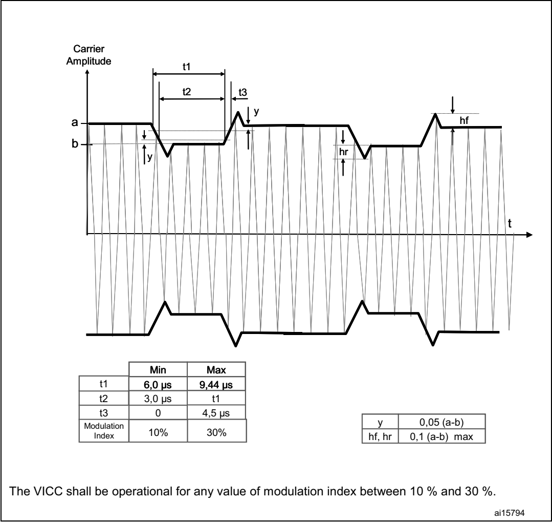
Figure 15. 10% modulation waveform
