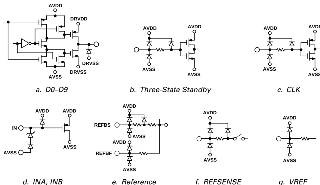
Figure 2. Equivalent Circuits
