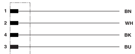
Contact assignment of the M5 connector
