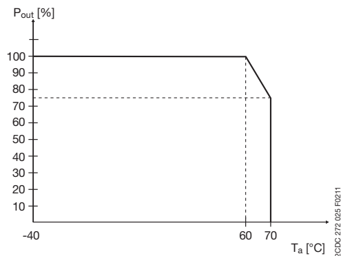
Fig. 5 Derating
