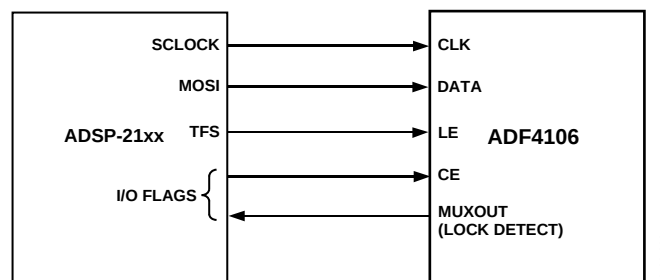
Figure 24. ADSP-21xx-to-ADF4106 Interface
