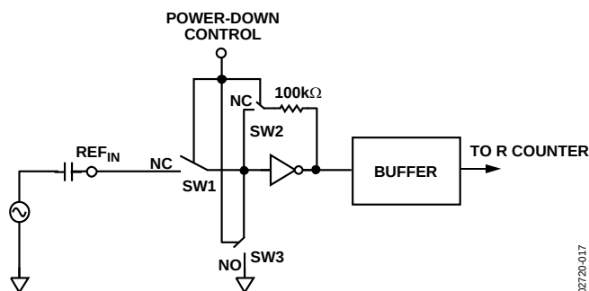
Figure 17. Reference Input Stage
