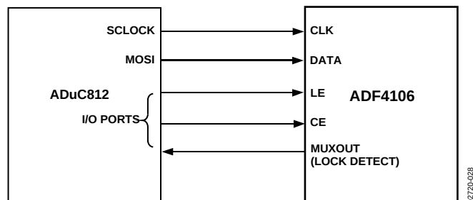
Figure 23. ADuC812-to-ADF4106 Interface
