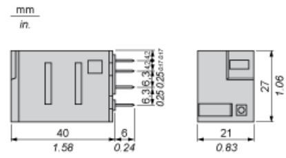
Pin Side View
